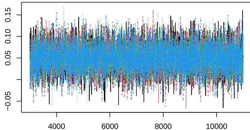
Trace of theta[3]
