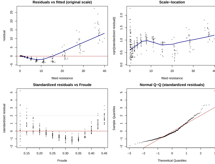
Figure 10: Original-scale residual diagnostics for the heteroscedastic nonlinear model M1, with each residual standardized by its own fitted standard deviation \hat{\sigma}_i = \hat{\sigma}_0 \hat{\mu}_i^\delta . Top left: raw residuals versus fitted resistance with a LOWESS trend (navy); the spread still fans out, the heteroscedasticity that the variance model must absorb. Top right: scale–location plot, \sqrt{|\text{standardized residual}|} versus fitted value; the roughly flat trend shows the learned variance function \sigma_i = \sigma_0 \mu_i^\delta removes the funnel. Bottom left: standardized residuals versus the Froude number with the \pm 2 reference band; no remaining trend against the physical driver. Bottom right: Normal Q–Q plot of the standardized residuals. After standardization the spread is close to unity and about 95% of points lie within \pm 2 , confirming that learning the variance corrects the heteroscedasticity.
