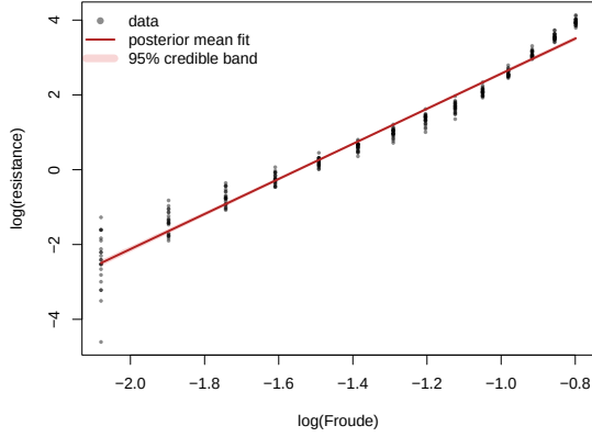
(a) Power-law fit on log-log axes.
