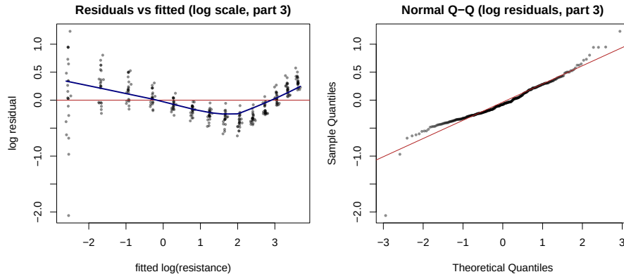
Figure 11: Log-scale residual diagnostics for the nonlinear model M1, plotted on the same axes as the part-1 log-log diagnostics (Fig. 6) for a like-for-like comparison. Left: log residuals \log y_i - \log \hat{\mu}_i versus the fitted log-resistance \log \hat{\mu}_i , with a LOWESS trend (navy). Right: Normal Q-Q plot of the log residuals. Because the learned variance is close to multiplicative ( \delta \approx 0.9 ), the M1 residuals are nearly homoscedastic on the log scale as well, mirroring the log-log fit; this is the log-lens counterpart of the agreement between \gamma_F \approx 4.82 and the log-log exponent \beta_F \approx 4.69 . The original-scale diagnostics (Fig. 10) remain the proper goodness-of-fit check for M1.
