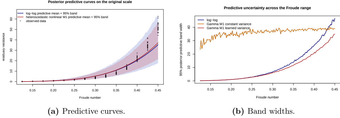
Figure 3: Posterior predictive comparison on the resistance scale. Left: fitted predictive bands and observed data. Right: interval width across Froude number.
