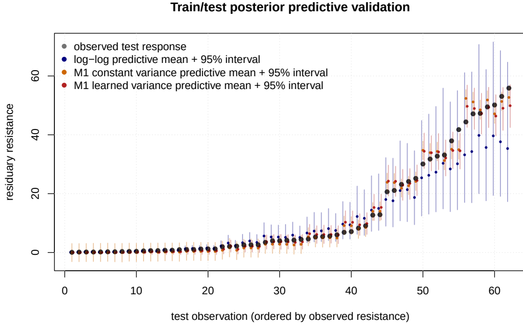
Figure 2: Train/test posterior predictive validation on the held-out rows. The black points are observed test responses ordered by resistance. Coloured points show posterior predictive means, and vertical intervals show the corresponding 95% posterior predictive bands for the log-log model, the constant-variance nonlinear M1 model, and the learned-variance nonlinear M1 model.
