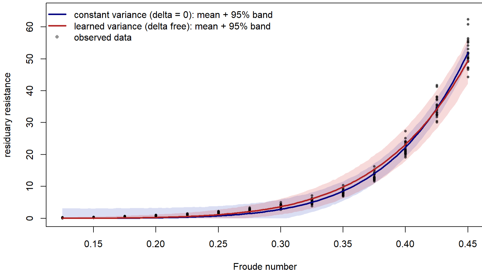
Posterior predictive: constant vs learned variance (Task 3)
