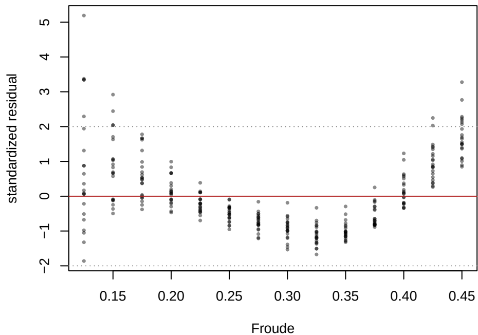
Standardized residuals vs Froude
