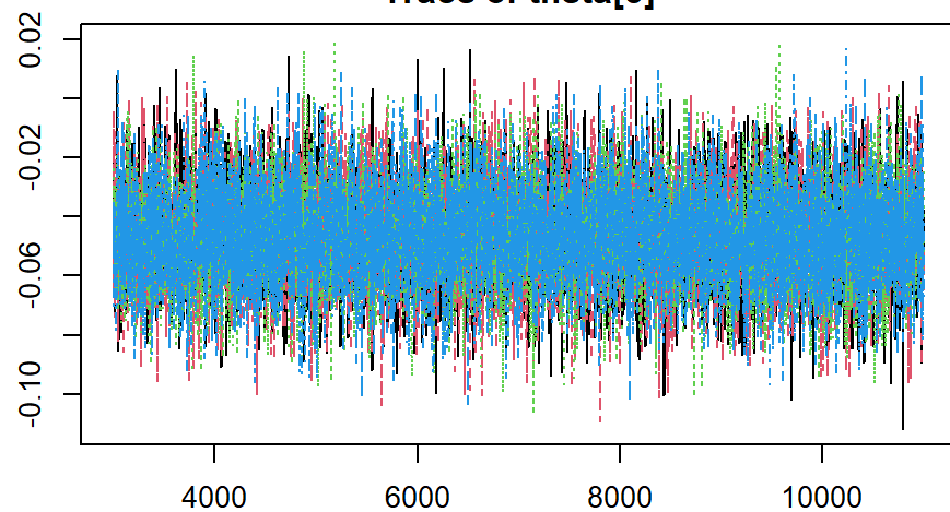
Trace of theta[3]
