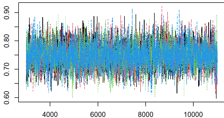
Trace of sigma0
