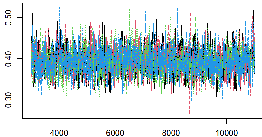
Trace of delta
