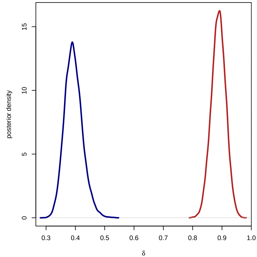
Likelihood sensitivity: \delta
