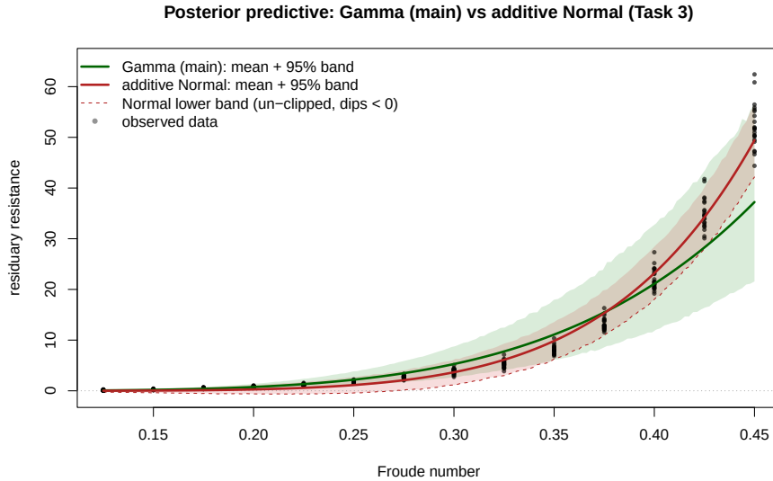
Figure 10: Posterior-predictive bands of the Gamma main model (green) and the additive-Normal sensitivity fit (red) on the original resistance scale, with observed data. The additive Normal's mean curve is steeper and its un-clipped lower band (dashed) dips below zero at low Froude, whereas the Gamma's lower band stays non-negative.
