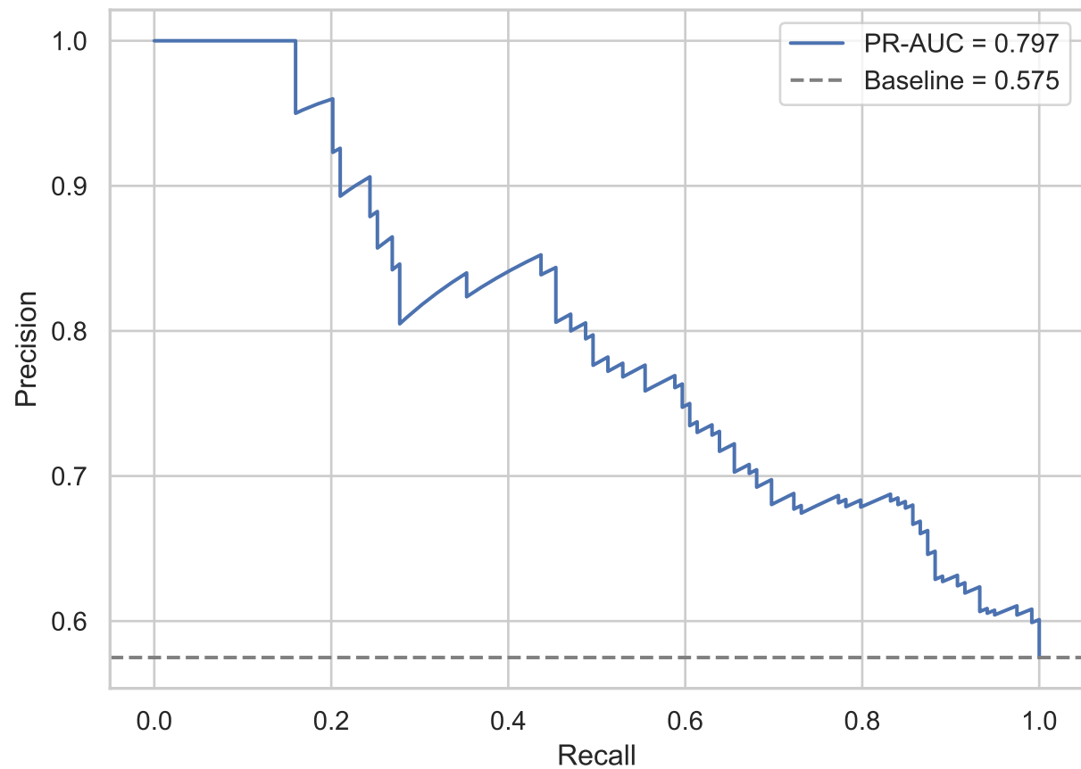
Precision-Recall - GAN reconstruction score
