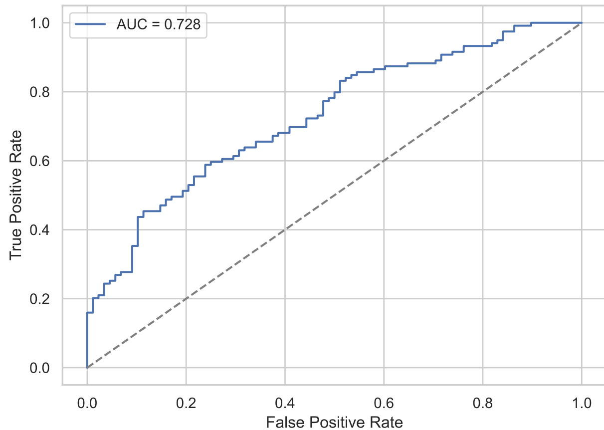
ROC - GAN reconstruction score
