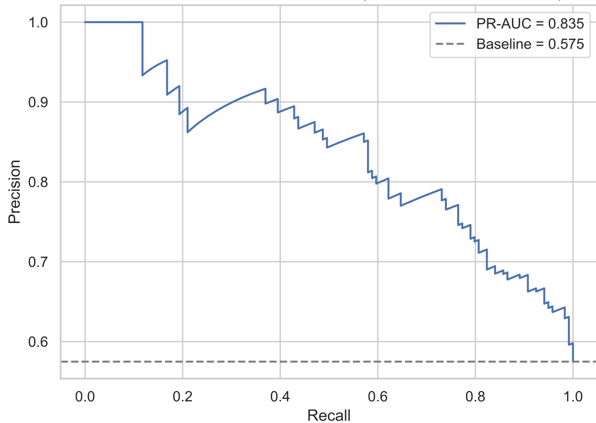
Precision-Recall - LSTM autoencoder (bidirectional + Mahalanobis)
