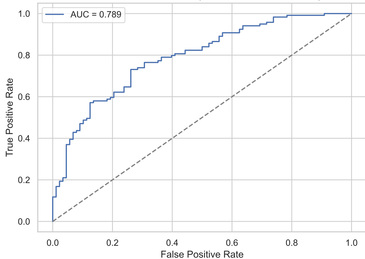
ROC - LSTM autoencoder (bidirectional + Mahalanobis)
