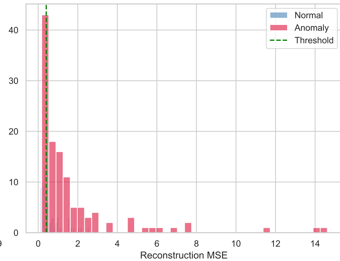
GAN reconstruction error
