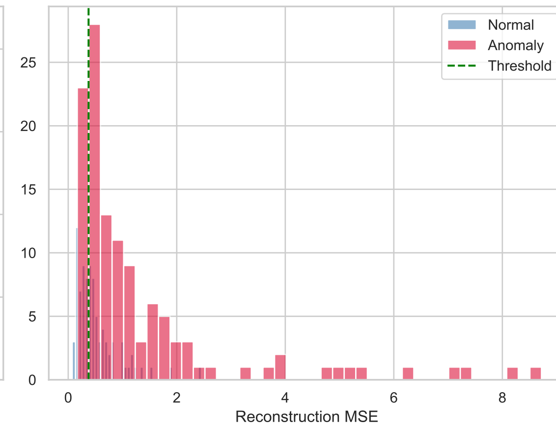
VAE reconstruction error
