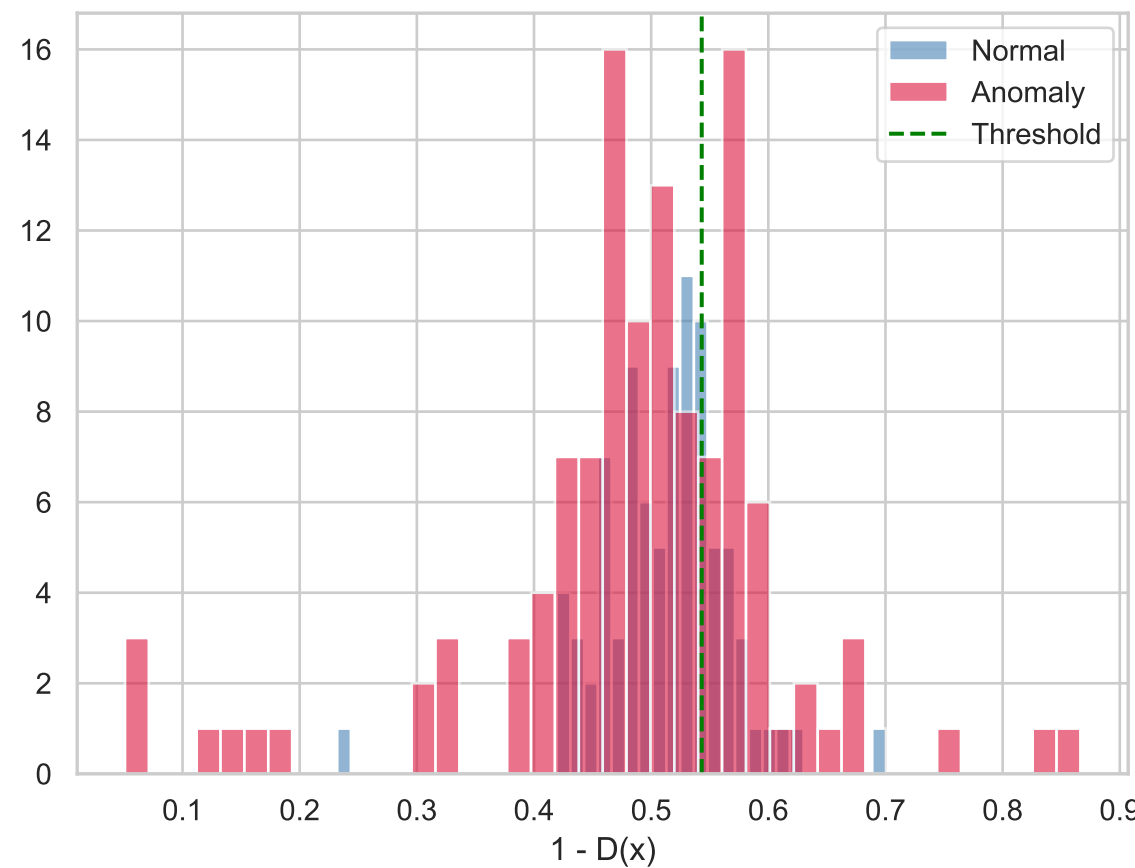
GAN discriminator: low realism is anomalous
