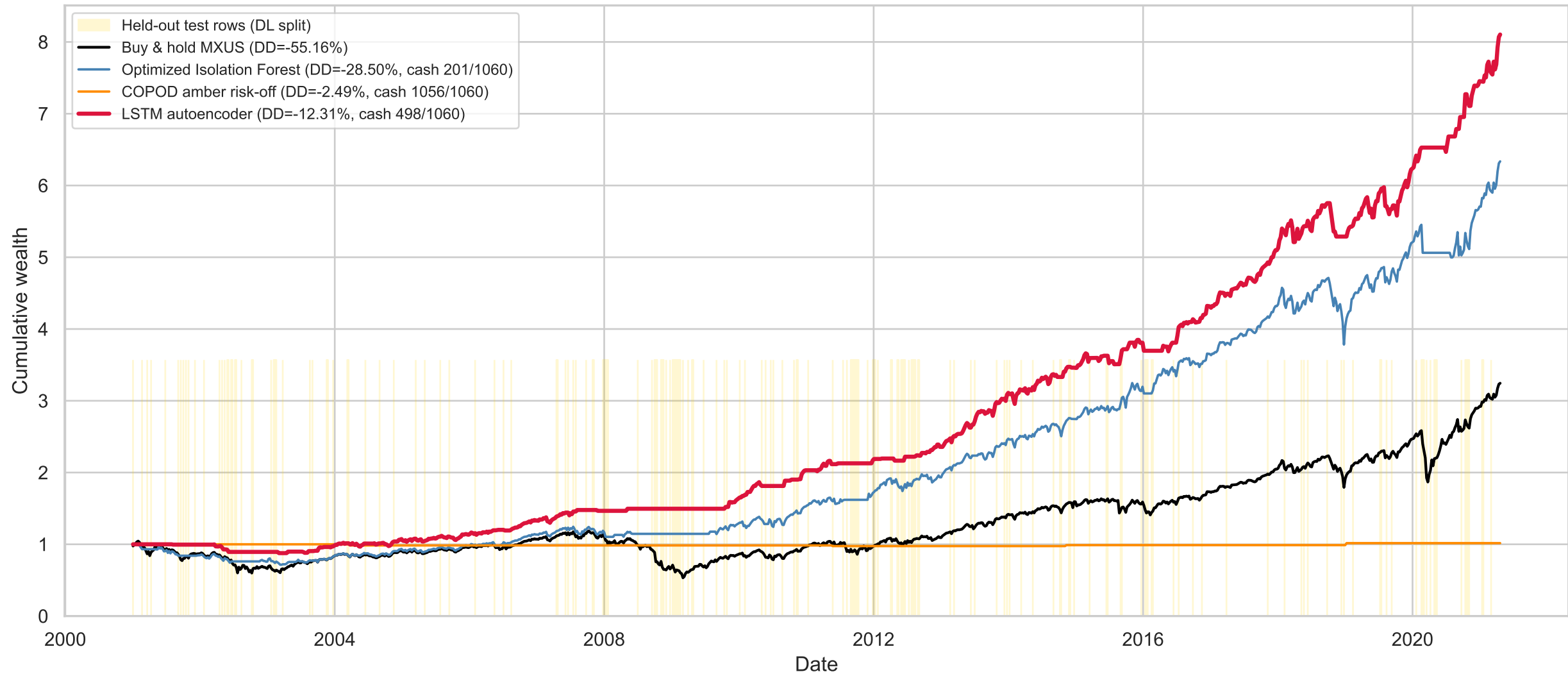
Cross-model risk-managed equity curves on a shared MXUS chronology (shaded = DL held-out test rows)
