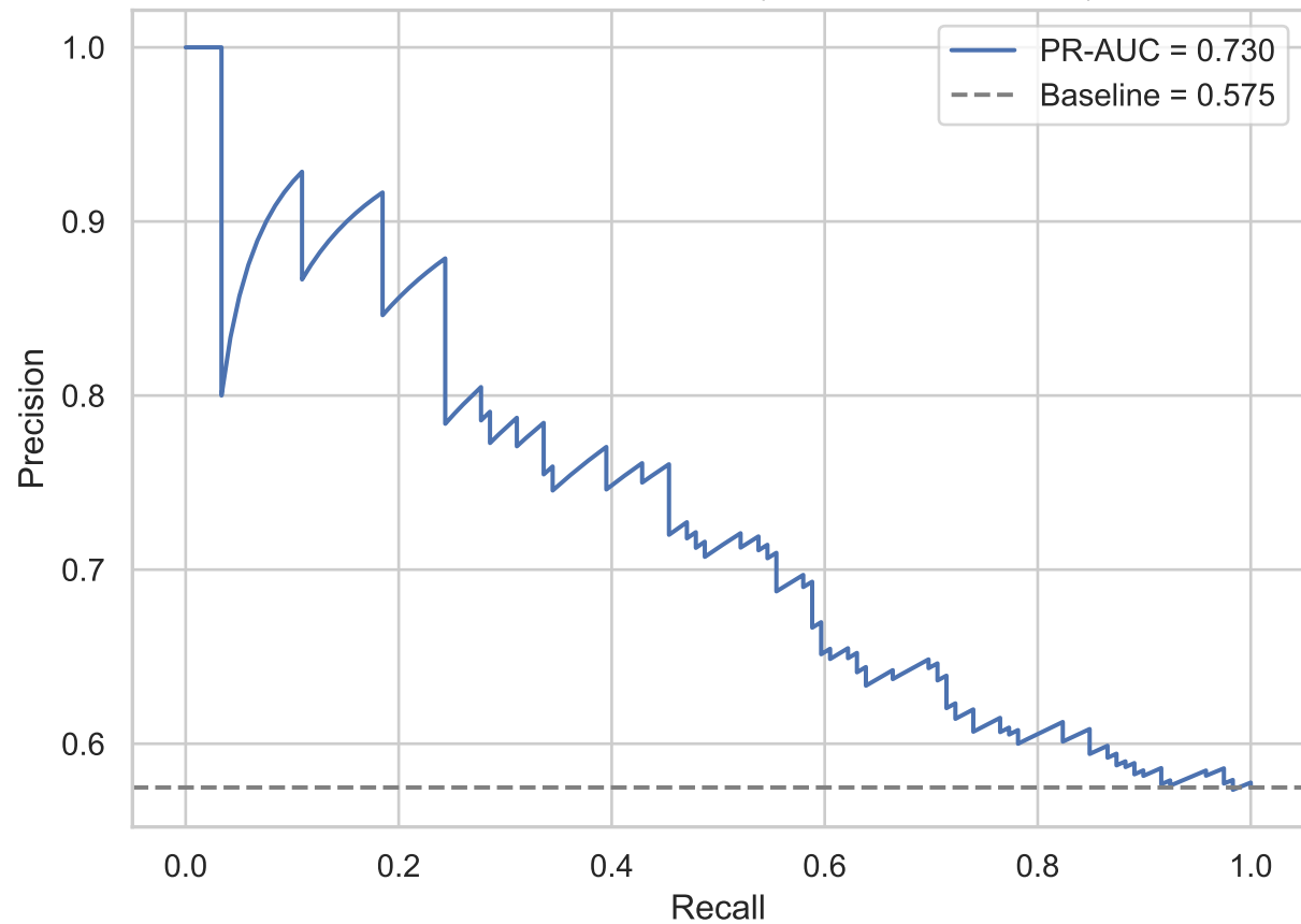
Precision-Recall - COPOD (Asset Grouped F-2.0)
