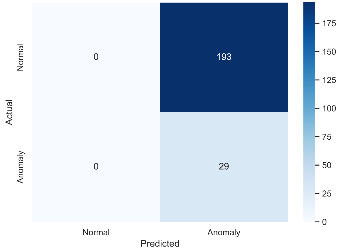
Confusion matrix - Grouped COPOD
