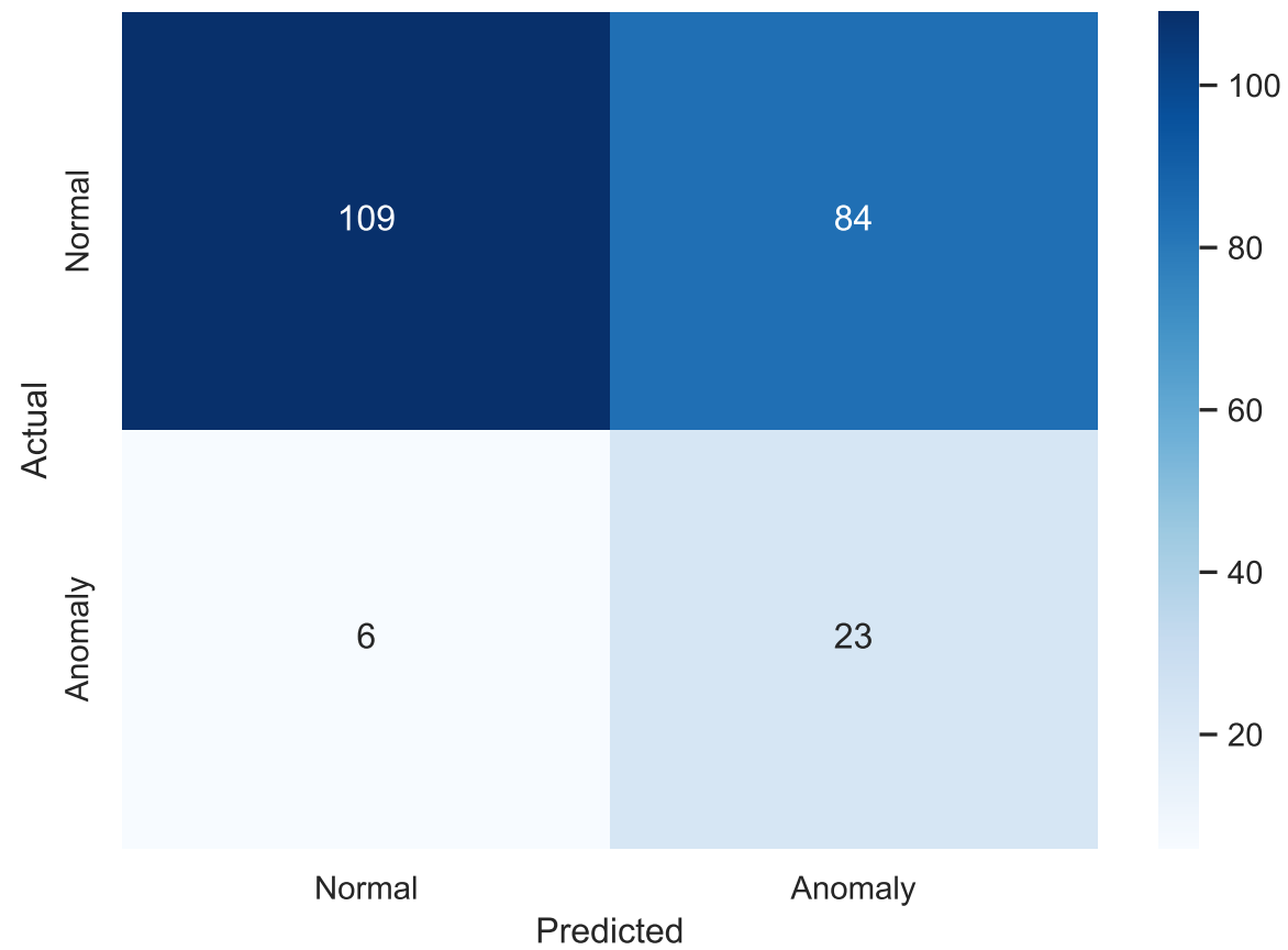
Confusion matrix - Isolation Forest
