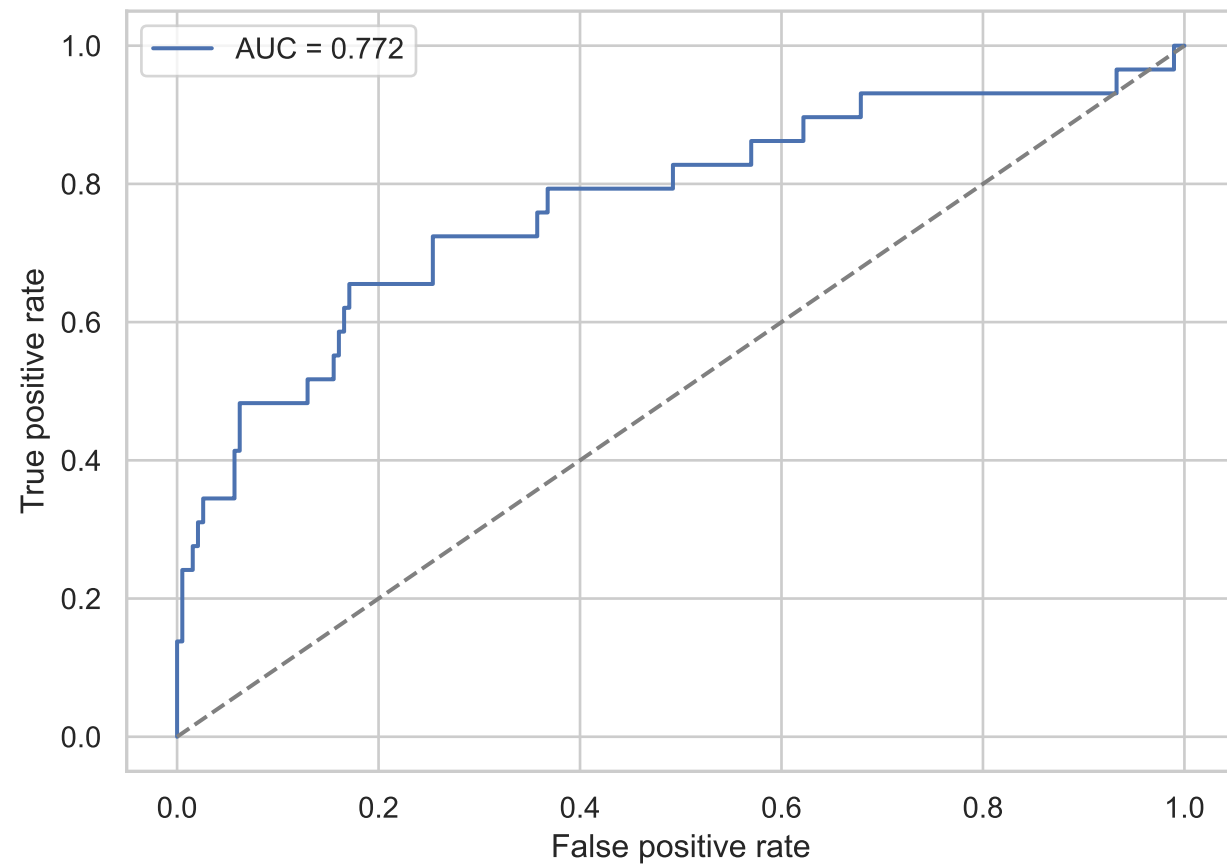
ROC - Isolation Forest
