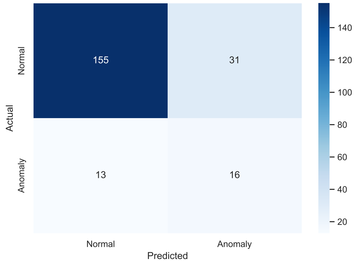
Confusion matrix - LSTM autoencoder
