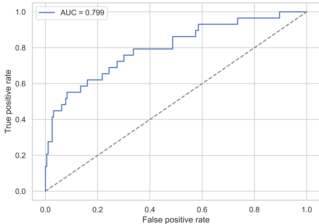
ROC - VAE reconstruction
