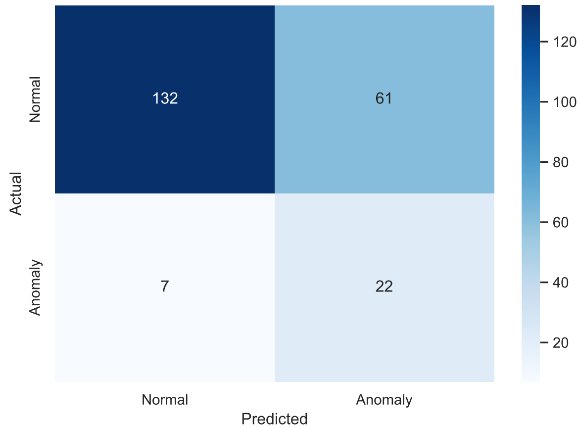
Confusion matrix - VAE reconstruction
