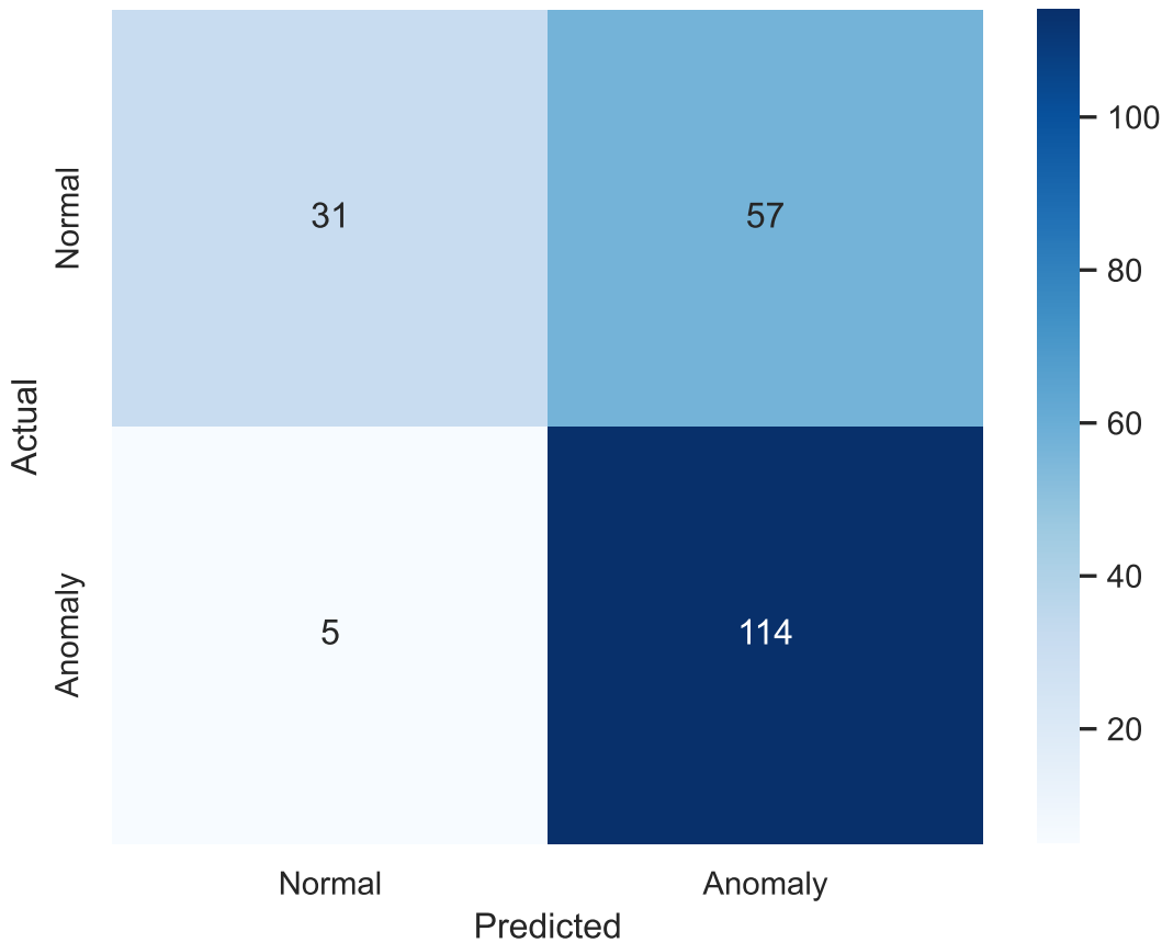
Confusion Matrix - LSTM autoencoder reconstruction score
