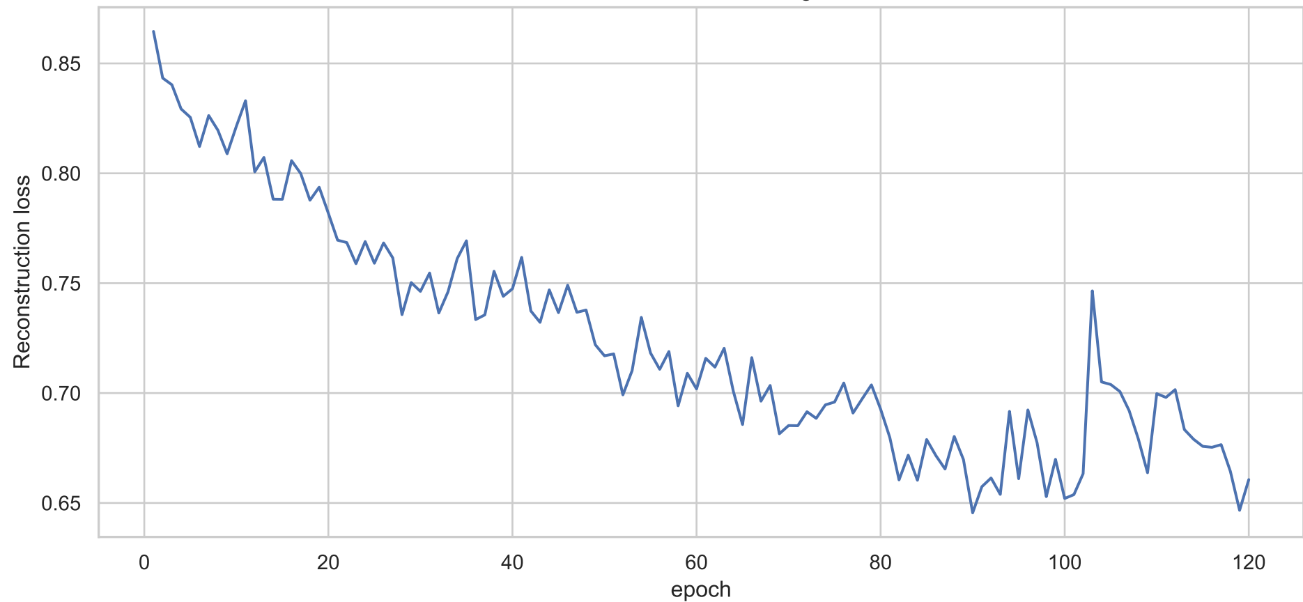
LSTM autoencoder training loss
