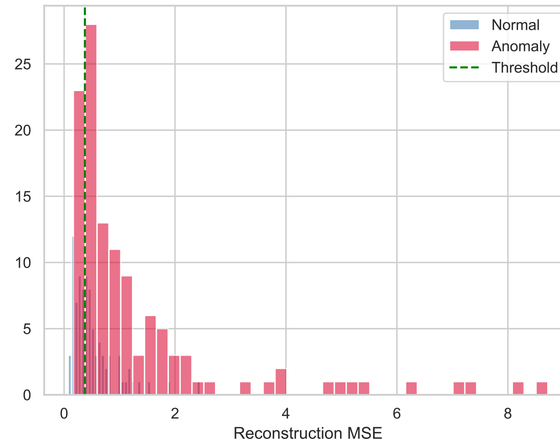
VAE reconstruction error
