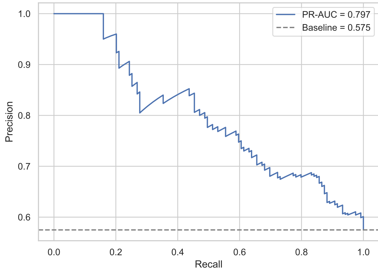
Precision-Recall - GAN reconstruction score
