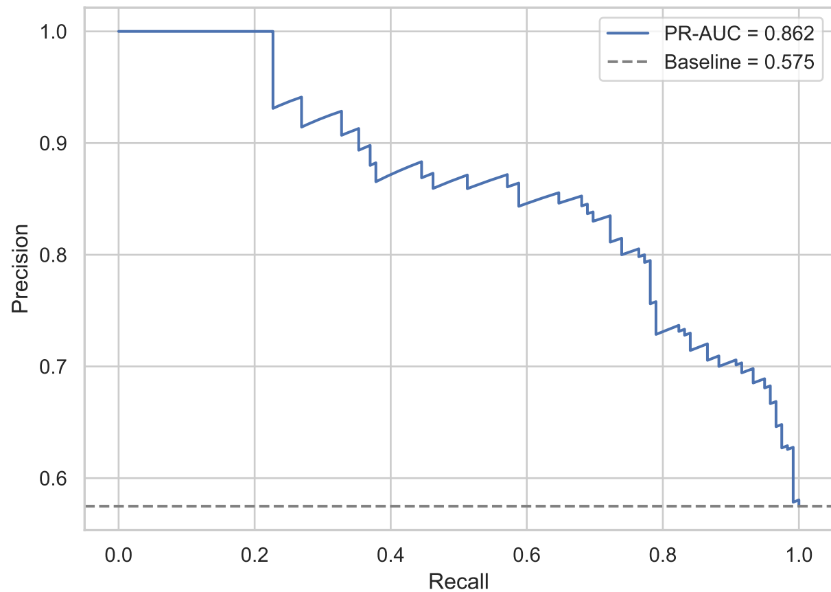
Precision-Recall - LSTM autoencoder reconstruction score
