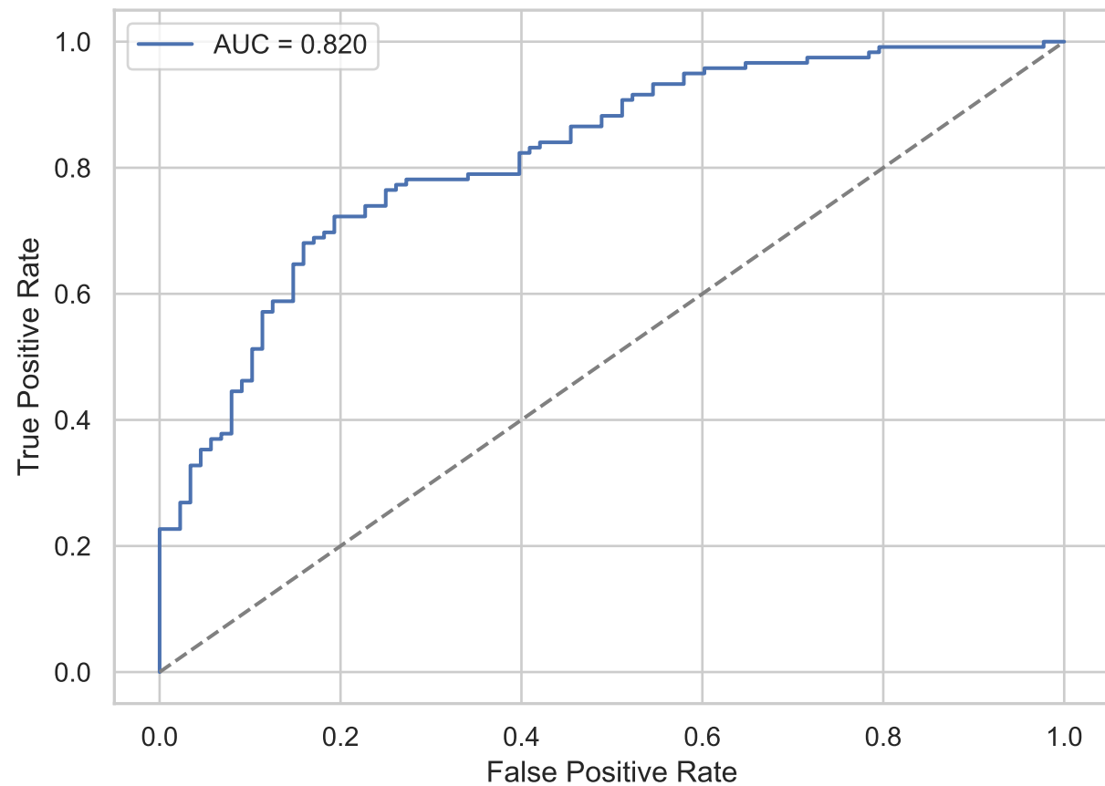
ROC - LSTM autoencoder reconstruction score
