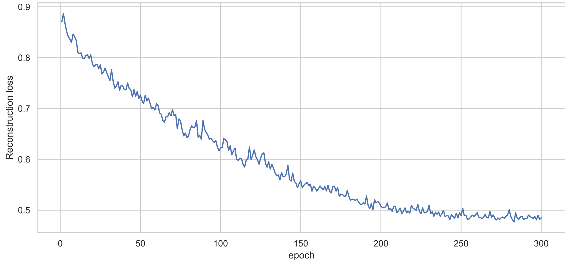
LSTM autoencoder training loss (bidirectional, 2-layer)
