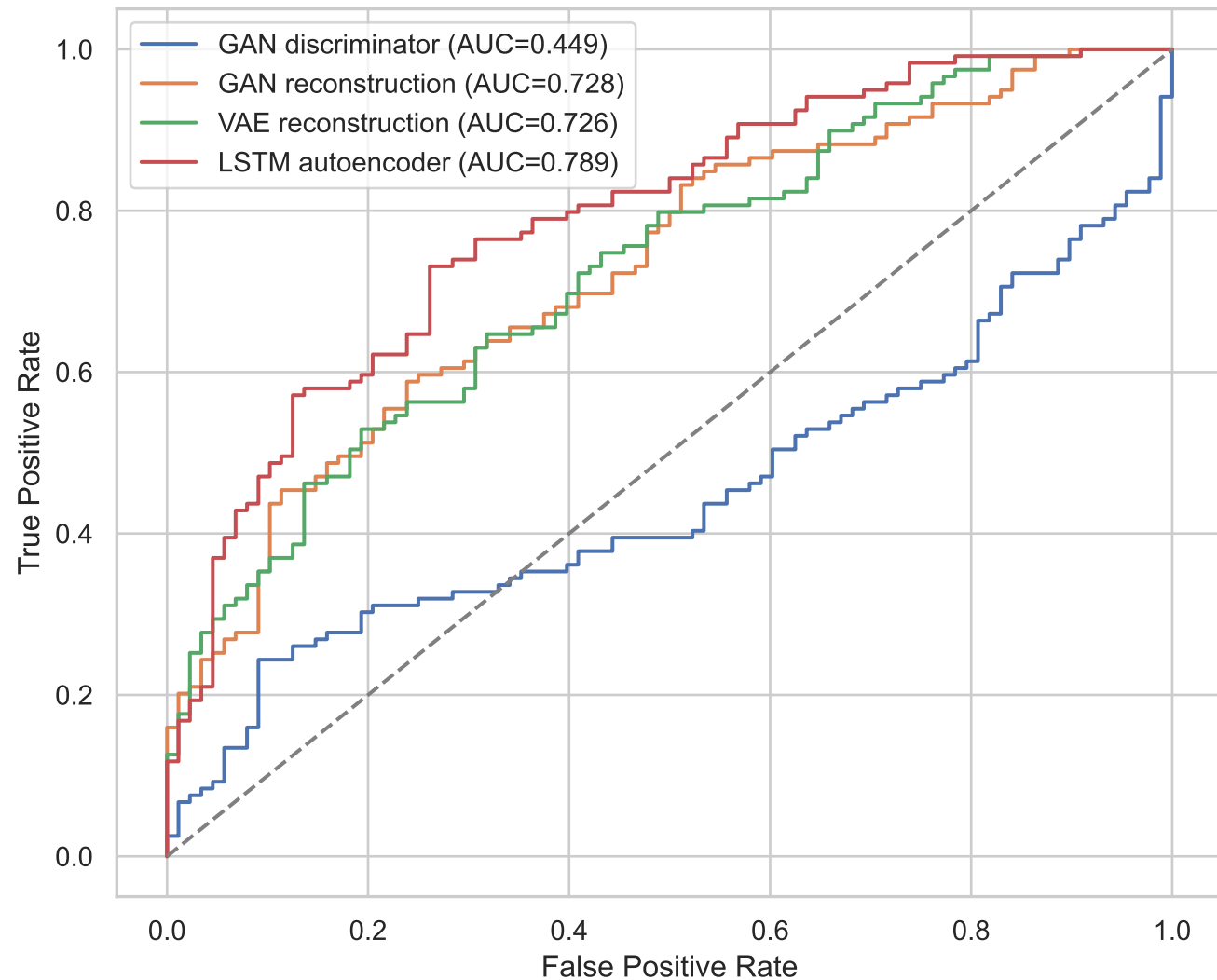
ROC comparison: GAN vs VAE vs LSTM
