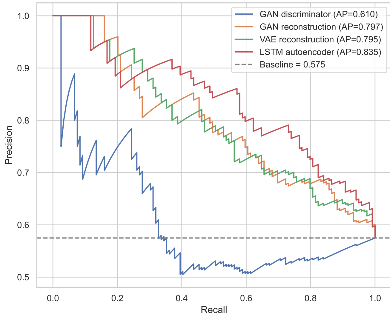
Precision-Recall: GAN vs VAE vs LSTM
