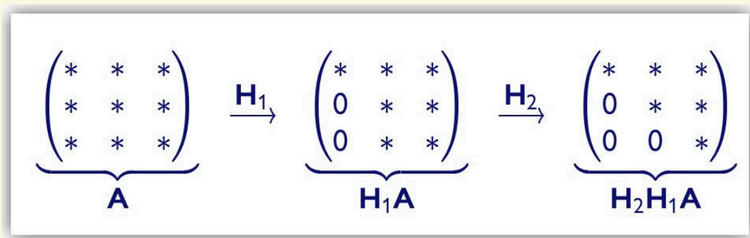
Figure 9.4: Householder QR factorization
