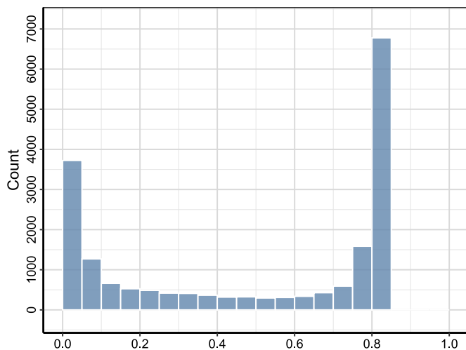
Posterior-PRPs (a) Histogram of posterior-PRPs
