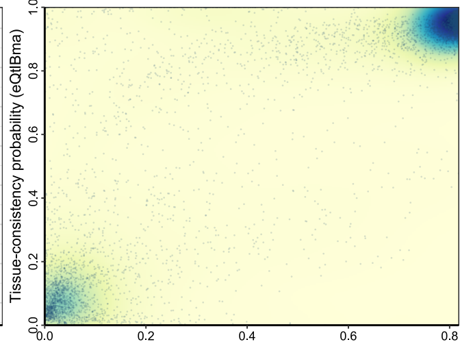
Posterior-PRPs (b) Smoothed scatter plot
