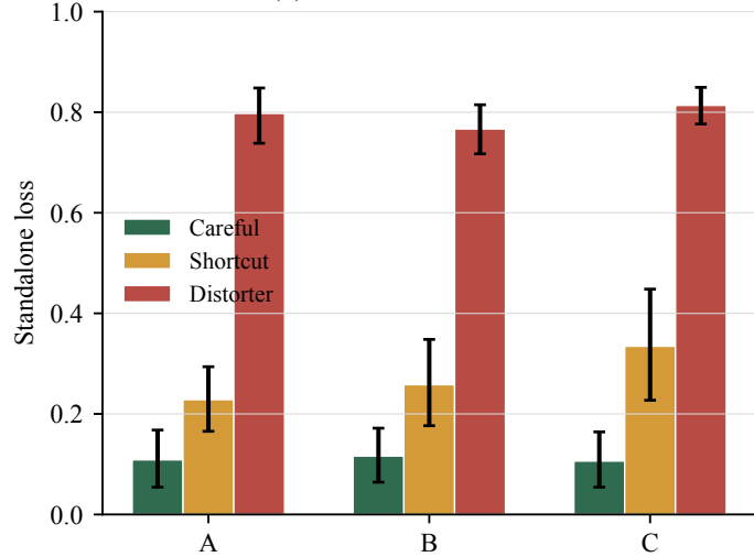
(a) LLM behavior modes
