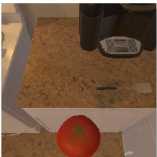
State 3
