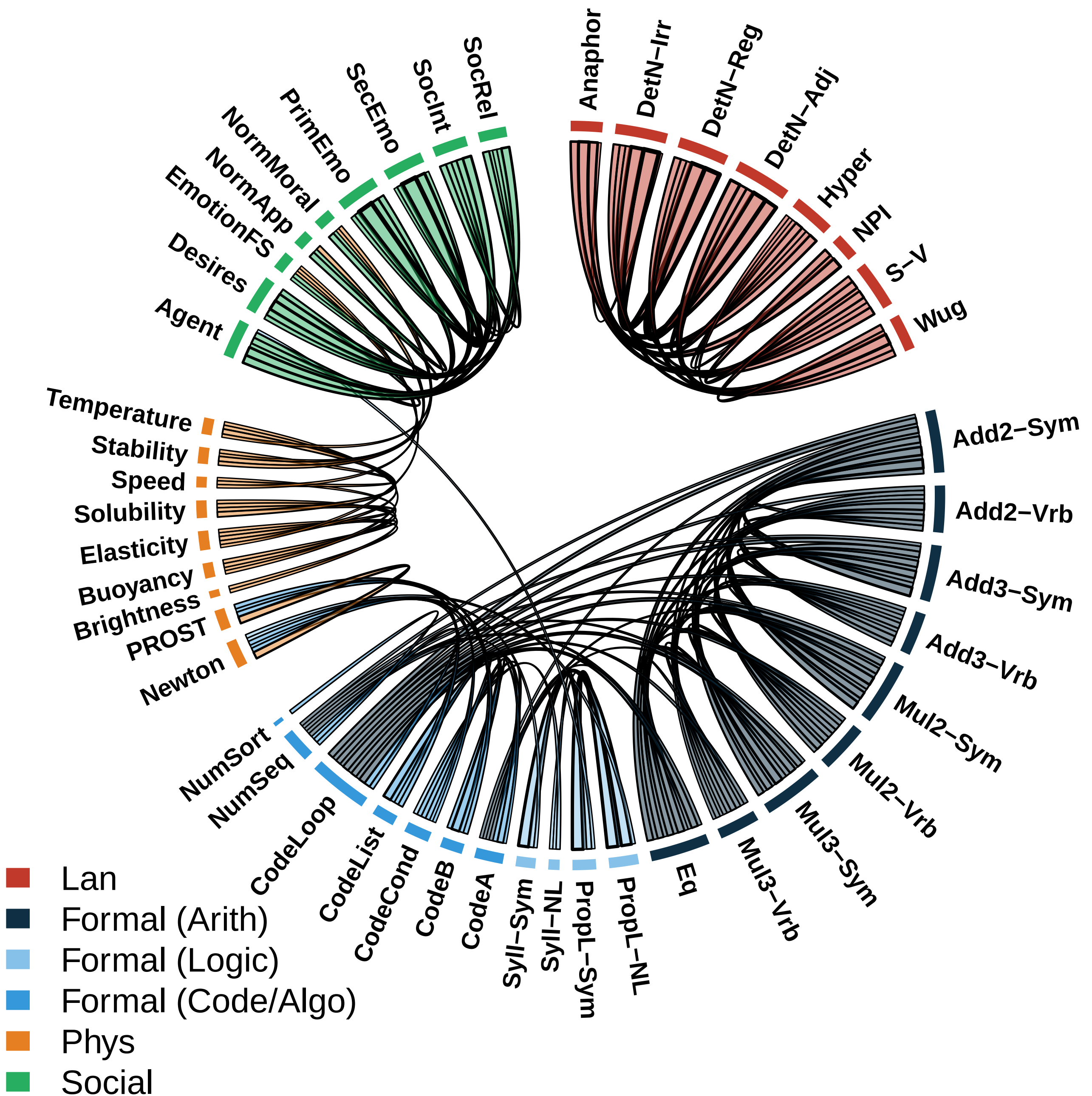
Cross-task neuron overlap (6-model average, top 0.1%, \geq 5\% )
