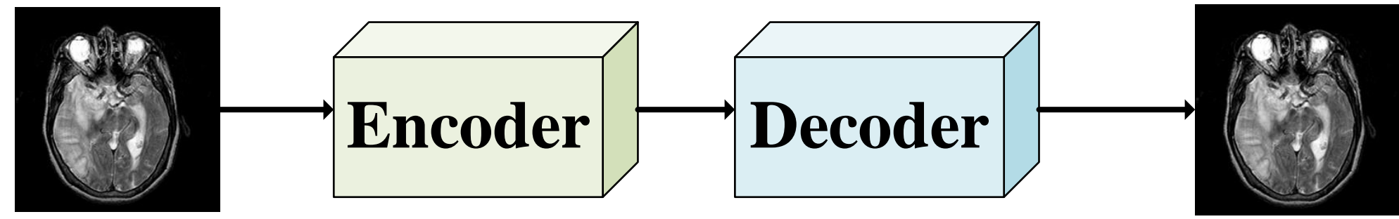
(a) Auto-Encoder
