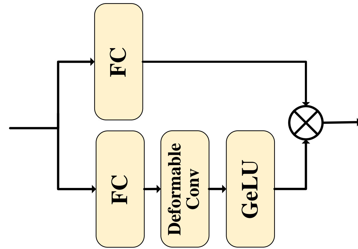
(b) Deformable Conv Gate Unit
