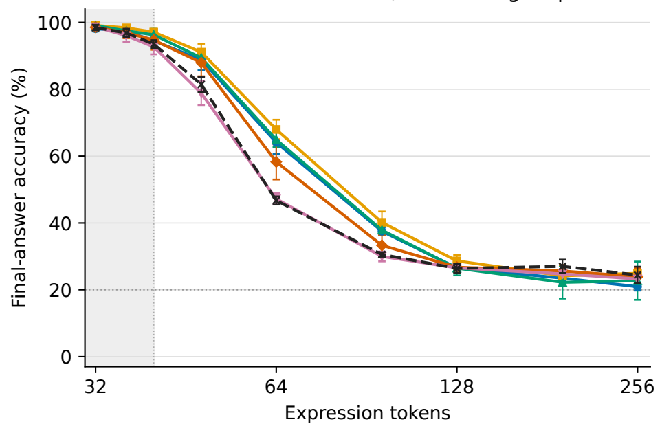
Mod-5 with brackets · 5,000 training steps
