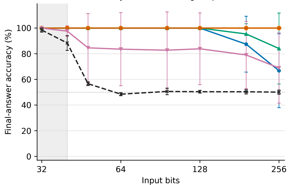
Parity · 2,000 training steps
