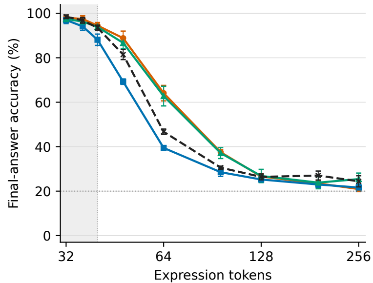
Mod-5 with brackets · 5,000 training steps
