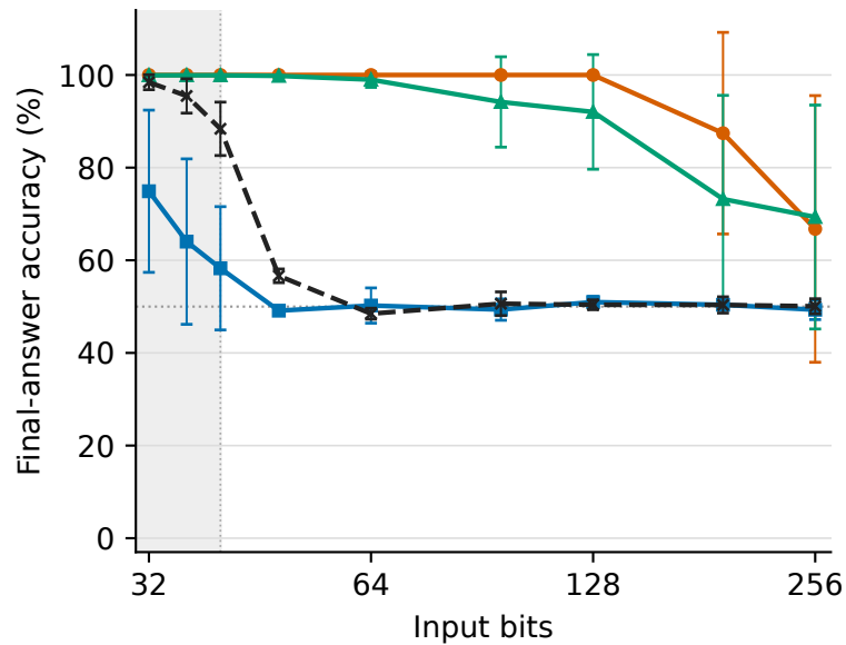
Parity · 2,000 training steps
