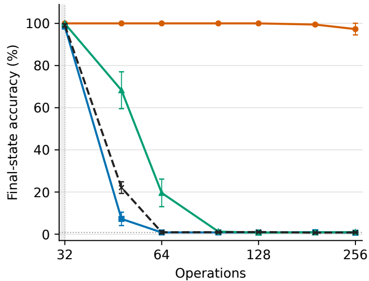
S_5 swaps · 2,000 training steps
