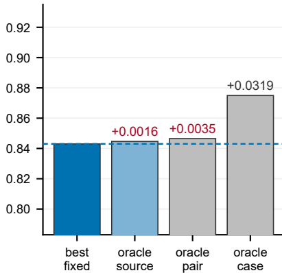
RIGA+ cup (best fixed: RandConv)
