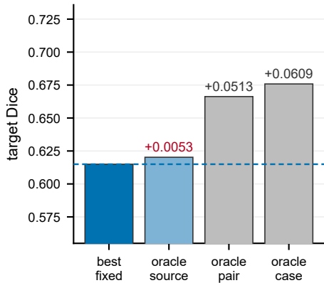
DG Prostate (best fixed: BigAug)
