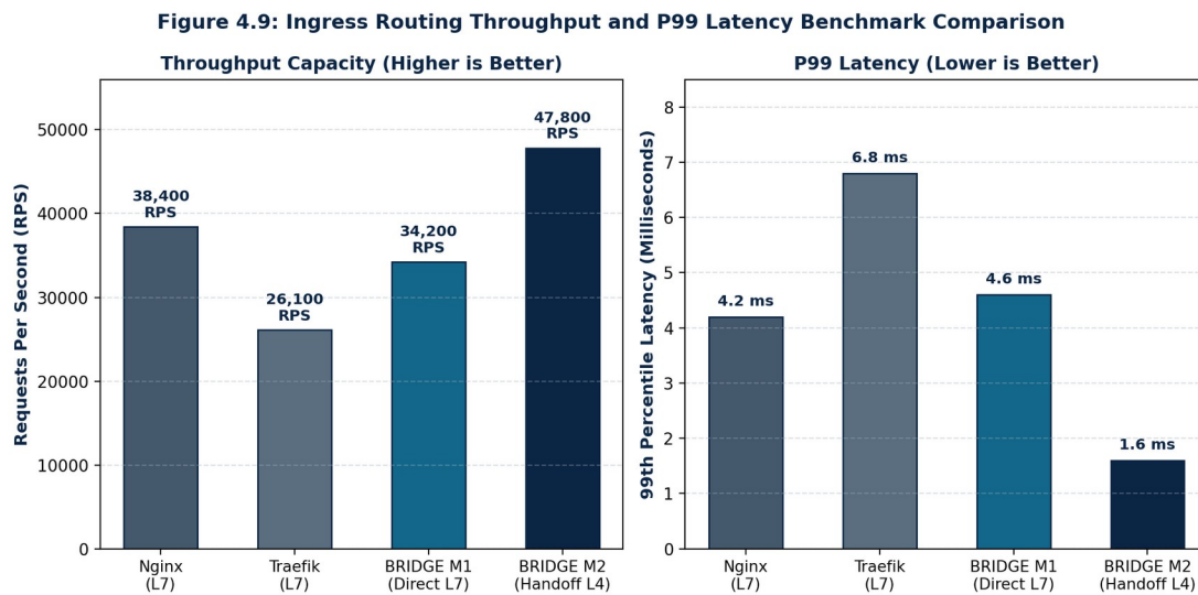
Figure 4.9: Ingress Routing Throughput and P99 Latency Benchmark Comparison
