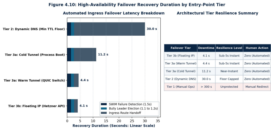
Figure 4.10: High-Availability Failover Recovery Duration by Entry-Point Tier
