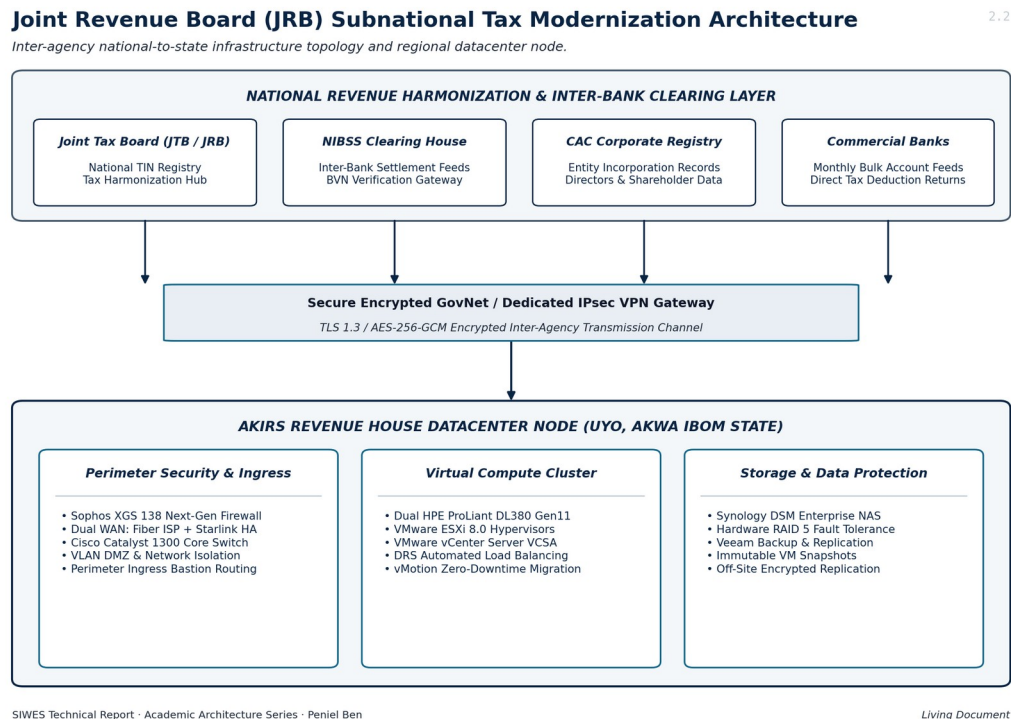
Figure 2.2: Joint Revenue Board (JRB) Subnational Tax Modernization Architecture
