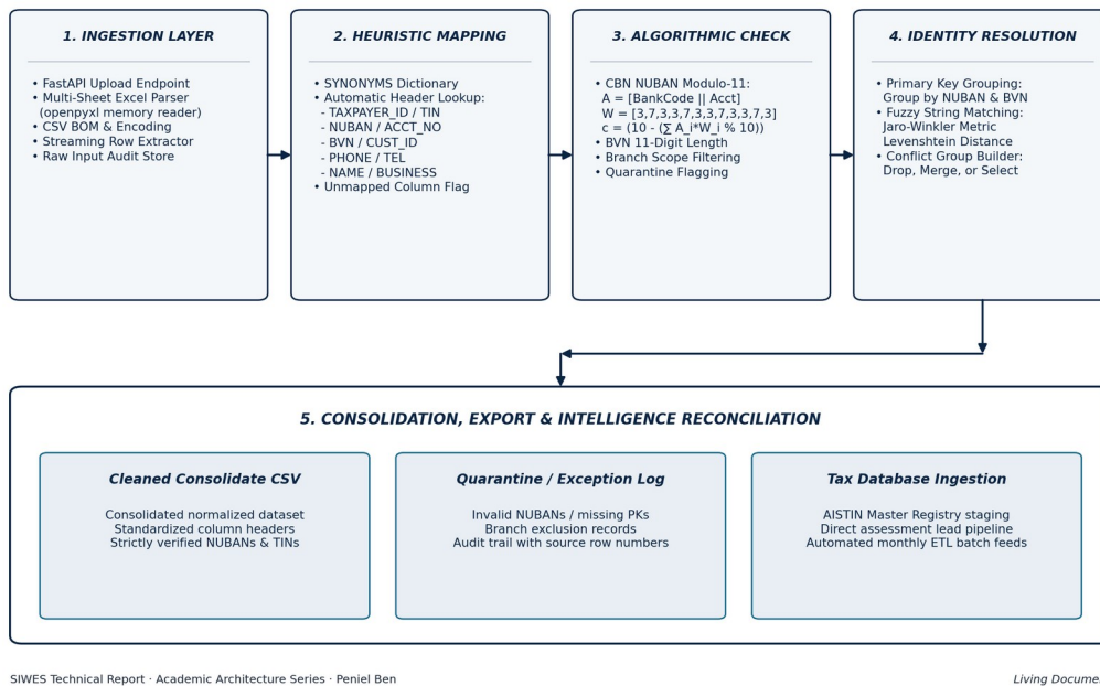
Figure 3.2: Automated Taxpayer Data Cleaning & Deduplication Pipeline Architecture
