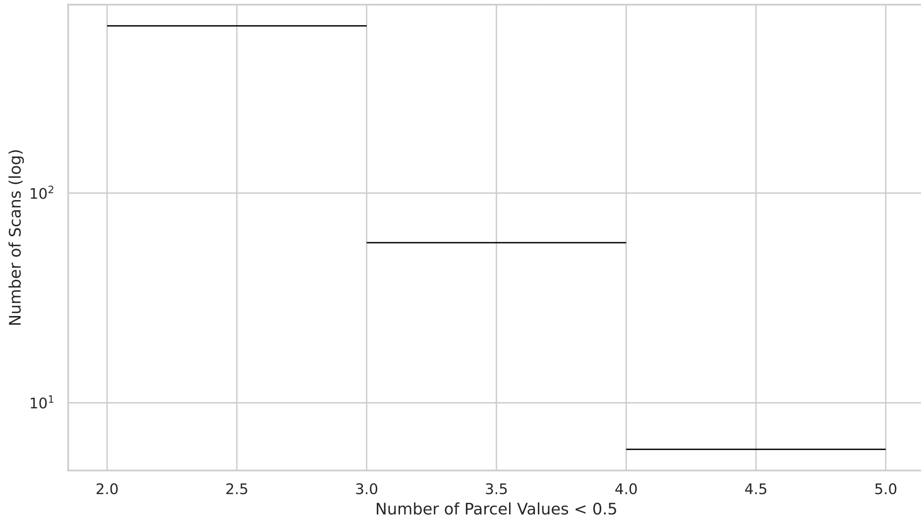
Histogram of Row Sum (Log-Scaled Y-Axis)
