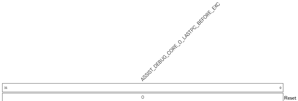
Register 17.30. ASSIST_DEBUG_CORE_0_LASTPC_BEFORE_EXCEPTION_REG (0x0094)
