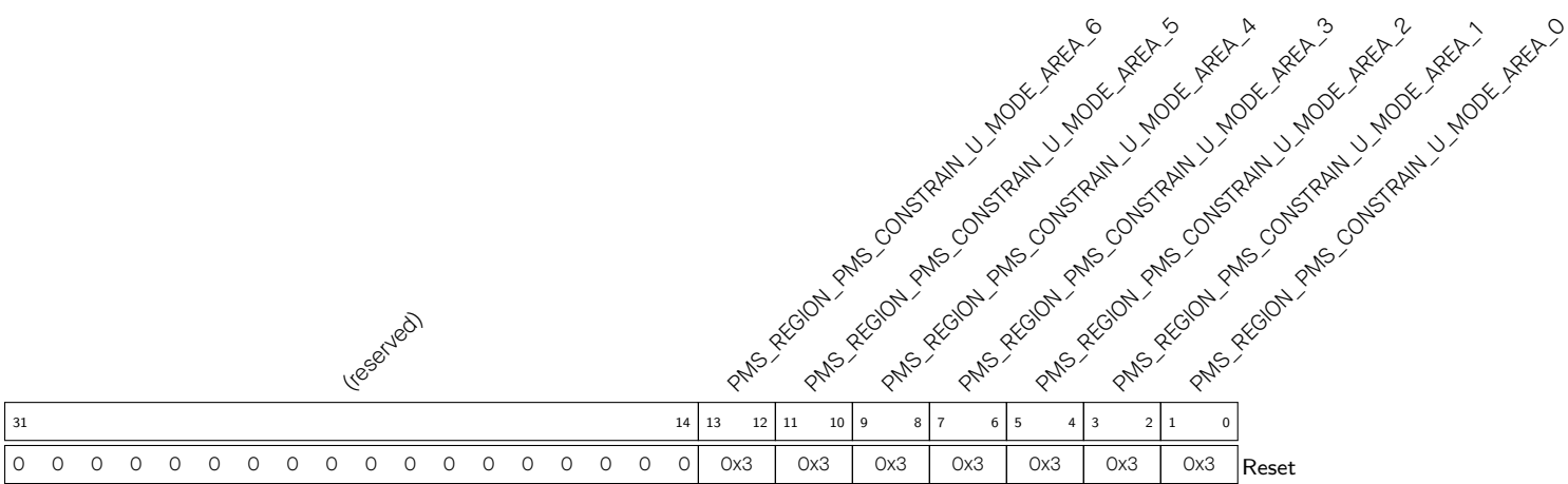
Register 14.50. PMS_REGION_PMS_CONSTRAIN_2_REG (0x010C)
