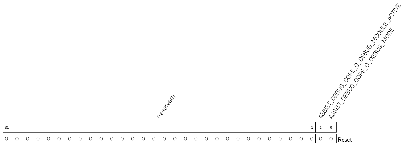
Register 17.31. ASSIST_DEBUG_CORE_0_DEBUG_MODE_REG (0x0098)
