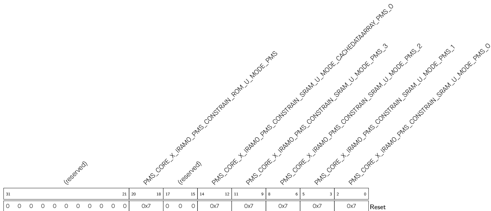
Register 14.29. PMS_CORE_X_IRAMO_PMS_CONSTRAN_1_REG (0x00AC)
