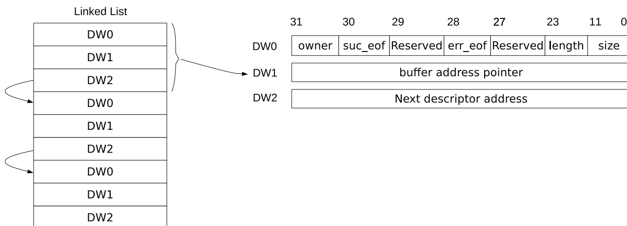
Figure 2.4-1. Structure of a Linked List
