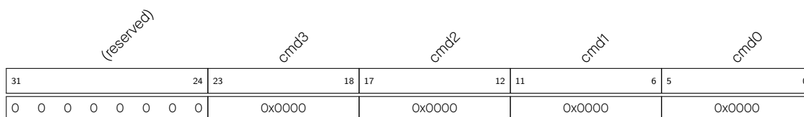
Figure 34.2-3. APB_SARADC_SAR_PATT_TAB1_REG and Pattern Table Entry 0 - Entry 3
