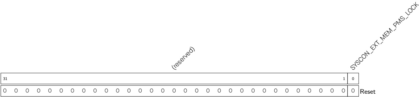
Register 14.73. SYSCON_EXT_MEM_PMS_LOCK_REG (0x0020)
