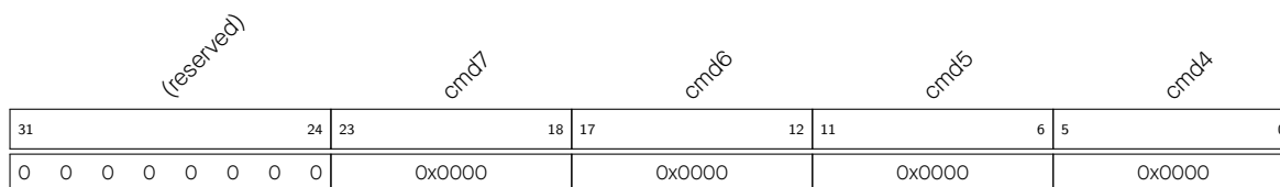
Figure 34.2-4. APB_SARADC_SAR_PATT_TAB2_REG and Pattern Table Entry 4 - Entry 7
