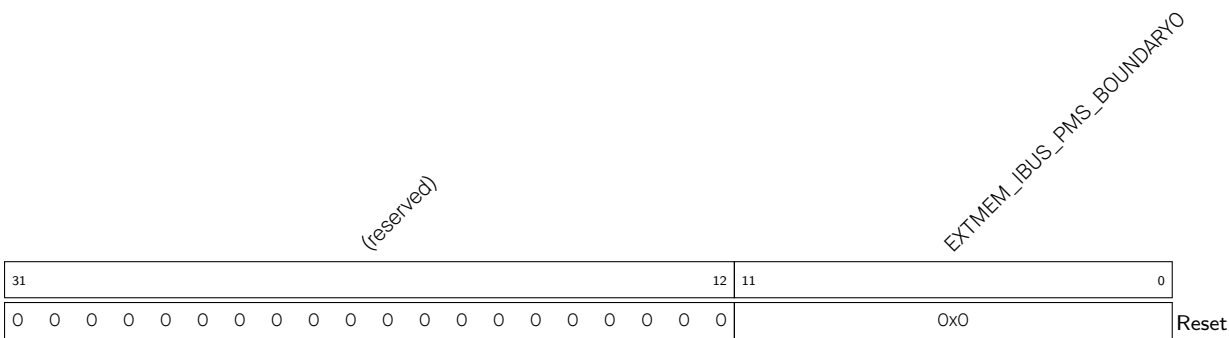
Register 14.80. EXTMEM_IBUS_PMS_TBL_BOUNDARY0_REG (0x00DC)
