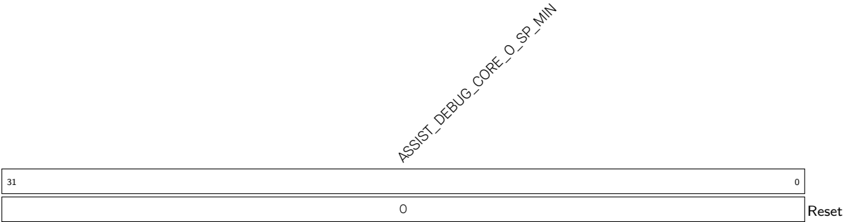
Register 17.12. ASSIST_DEBUG_CORE_O_SP_MIN_REG (0x0038)
