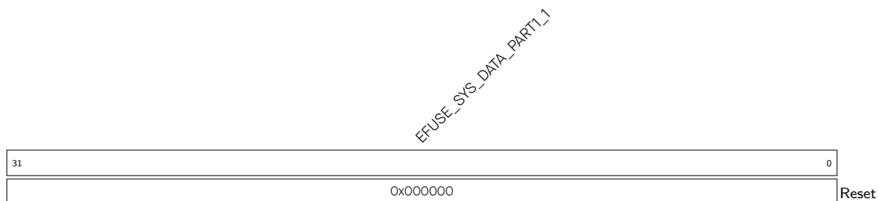
Register 4.25. EFUSE_RD_SYS_PART1_DATA1_REG (0x0060)
