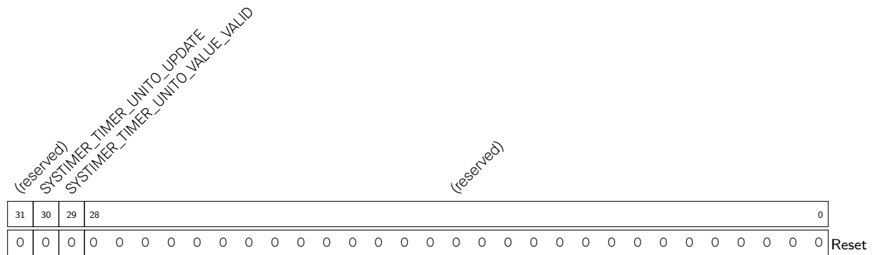
Register 10.2. SYSTIMER_UNIT0_OP_REG (0x0004)
