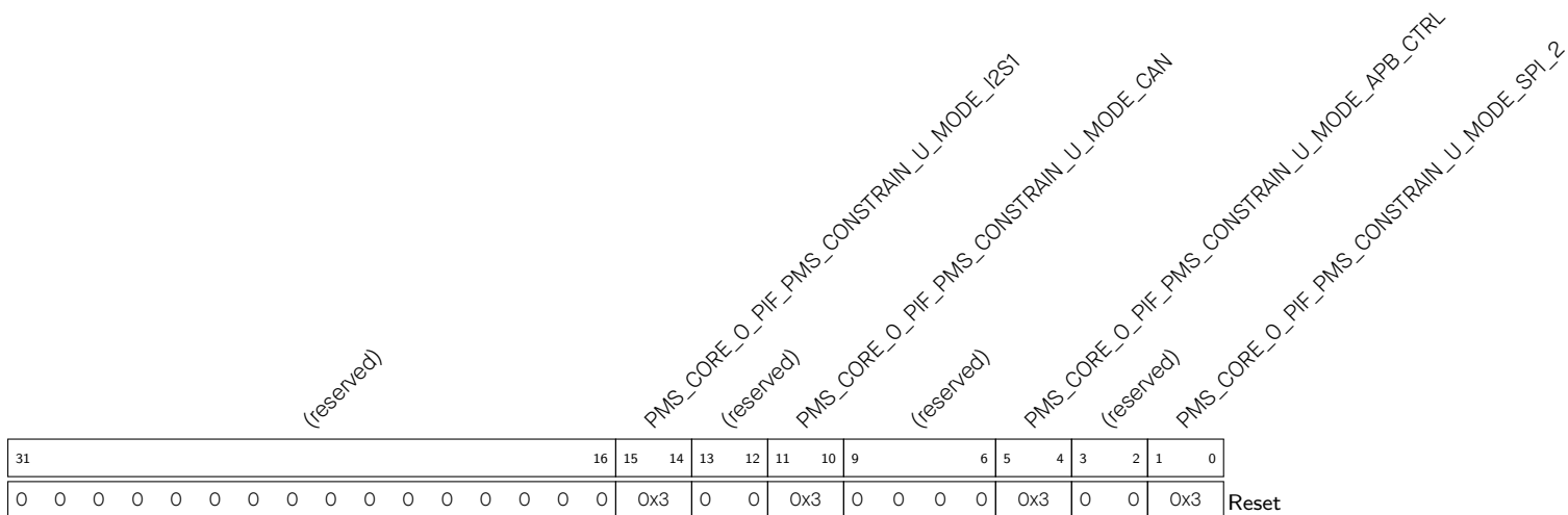
Register 14.44. PMS_CORE_O_PIF_PMS_CONSTRRAIN_7_REG (0x00F4)
