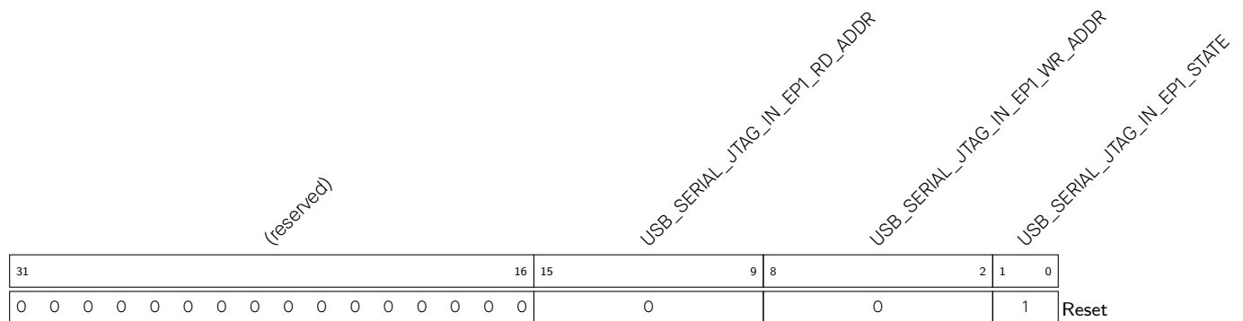
Register 30.10. USB_SERIAL_JTAG_IN_EP1_ST_REG (0x002C)
