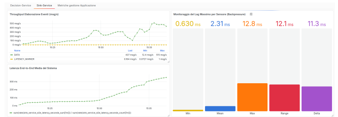
Fig. 10. Metriche Sink-service.
