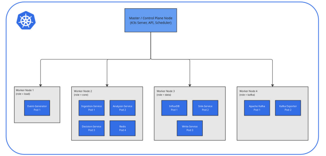
Fig. 4. Cluster K3s.
