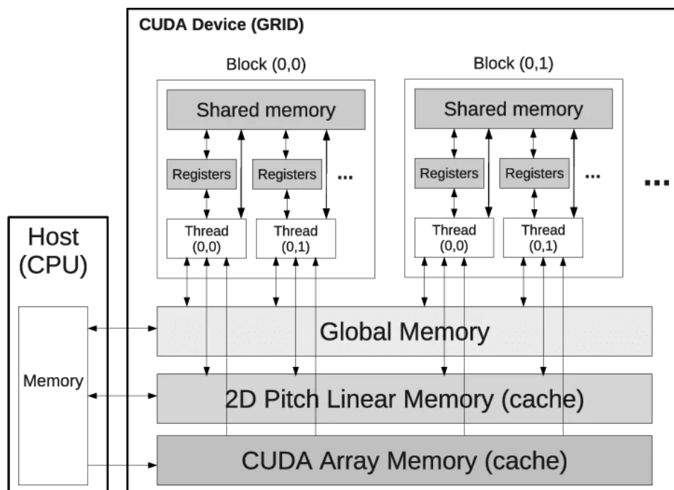
Figura 2.7: Modelo host-device de CUDA [Sanchez and Rodriguez, 2013]
