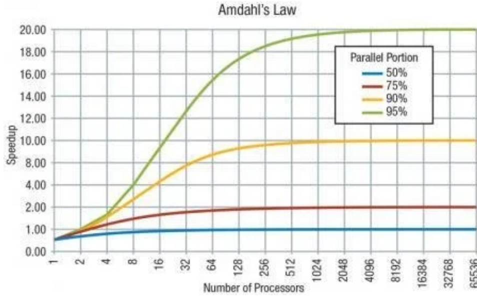
Figura 2.3: Ley de Amdahl [Shiang et al., 2016]
