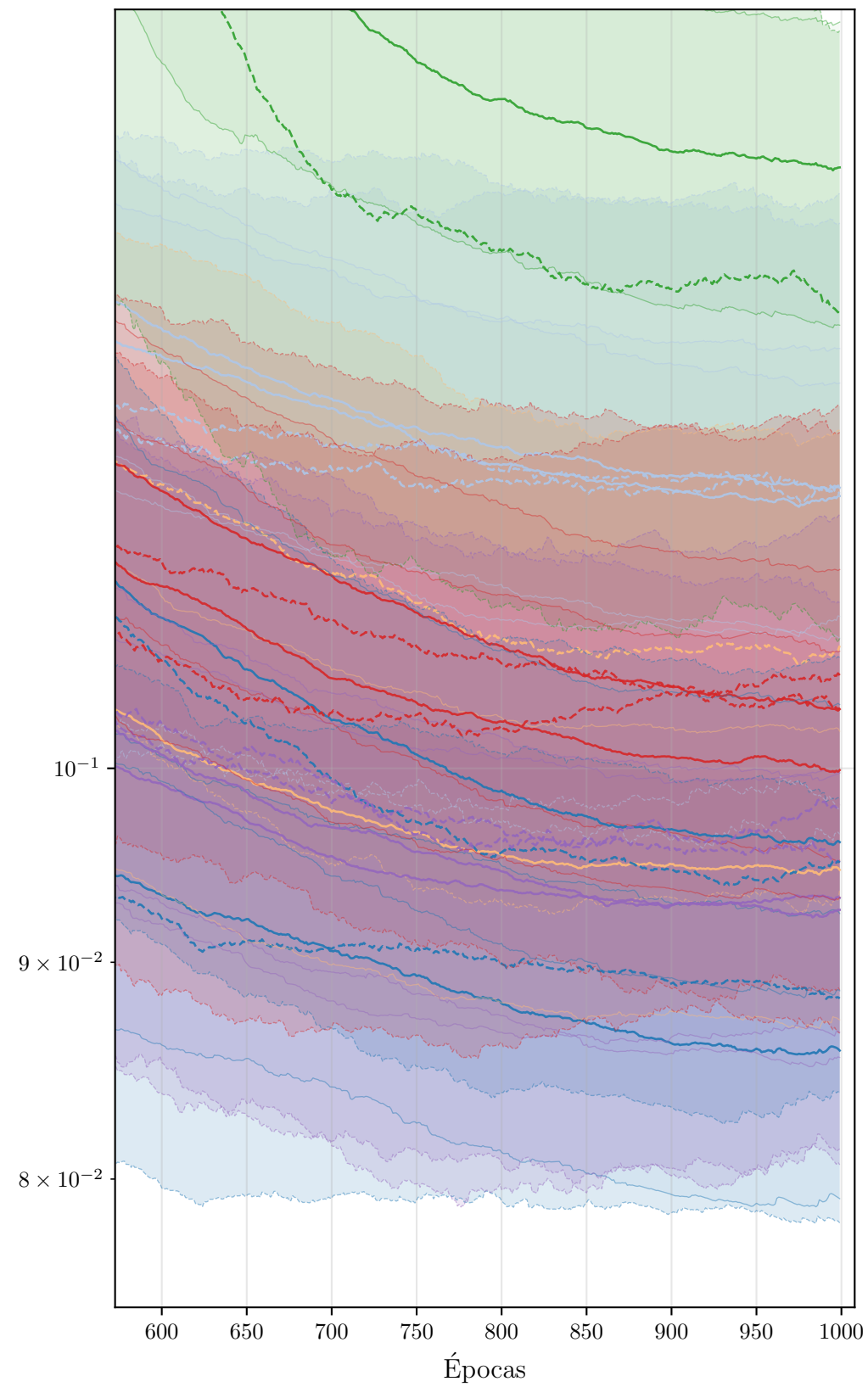
Loss
