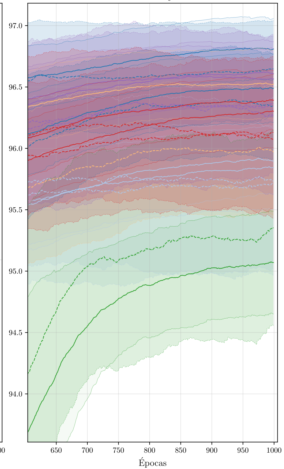
Accuracy
