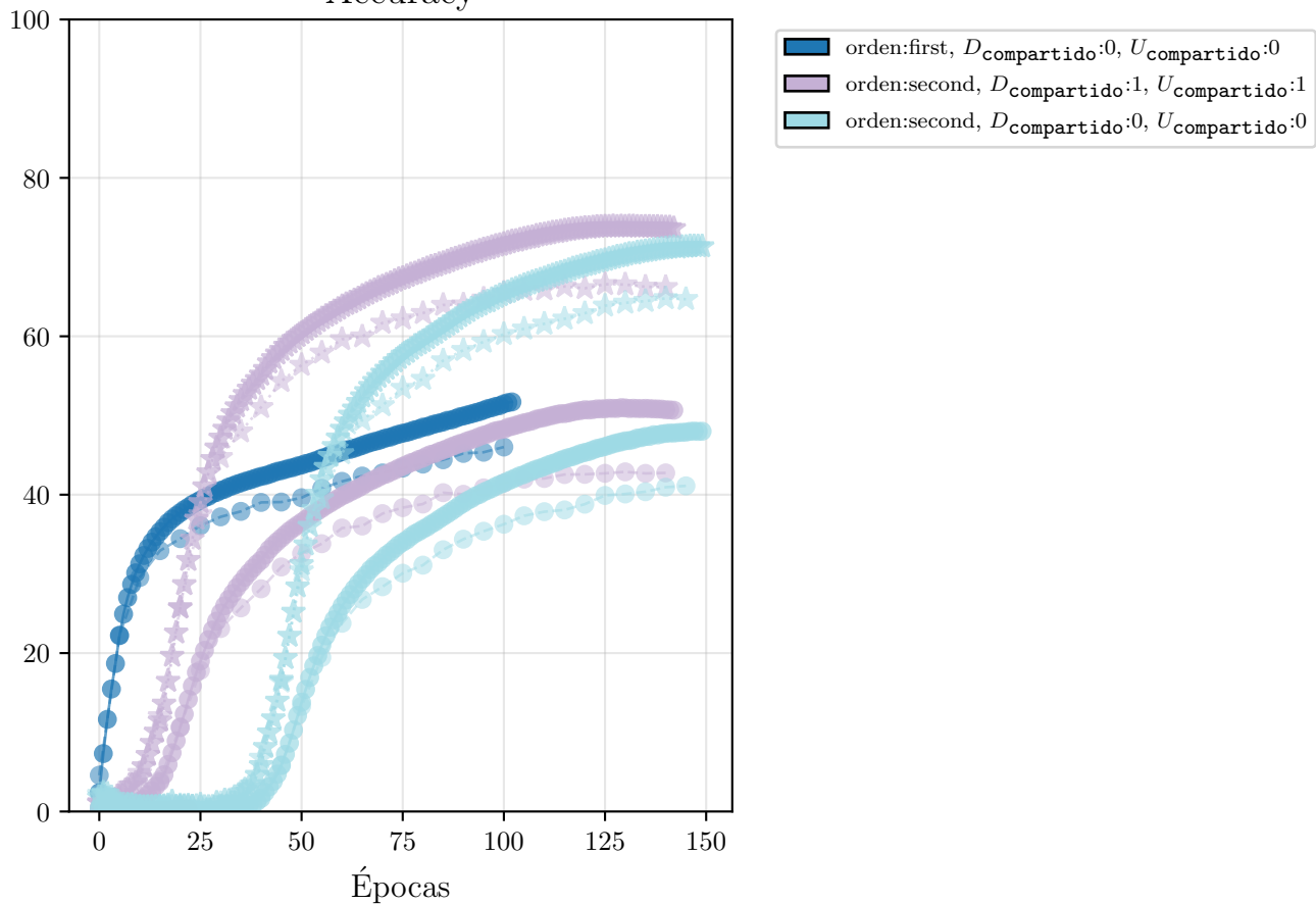
Accuracy
