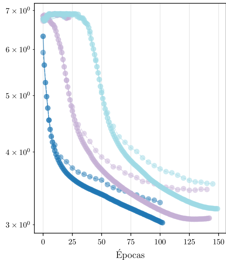
Loss
