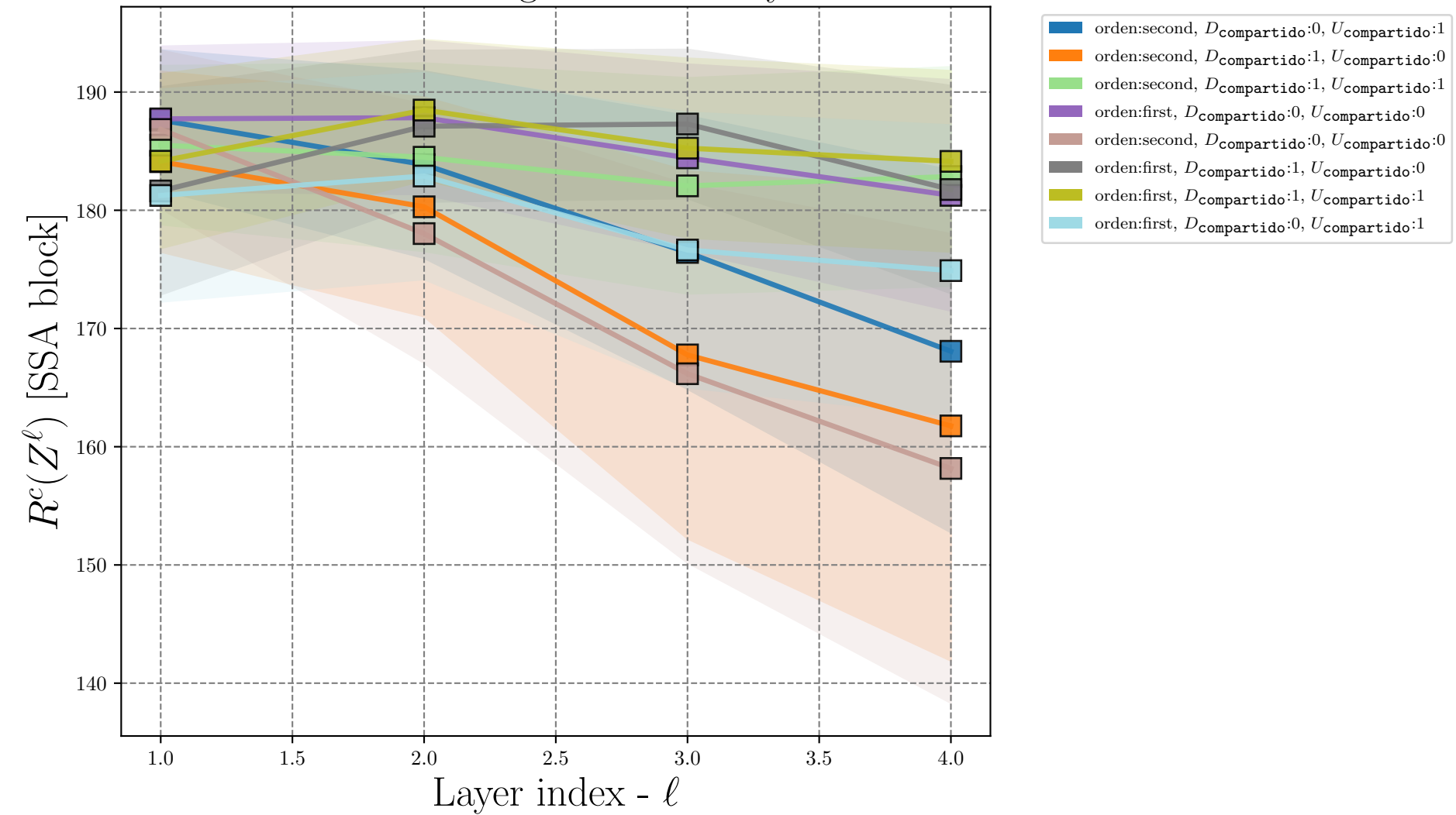
Measure coding rate across layers
