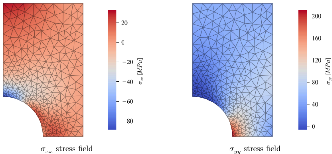
Figure 11: Horizontal and vertical stresses from the textbook
