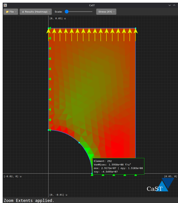
Figure 13: Shearing stress heatmap
