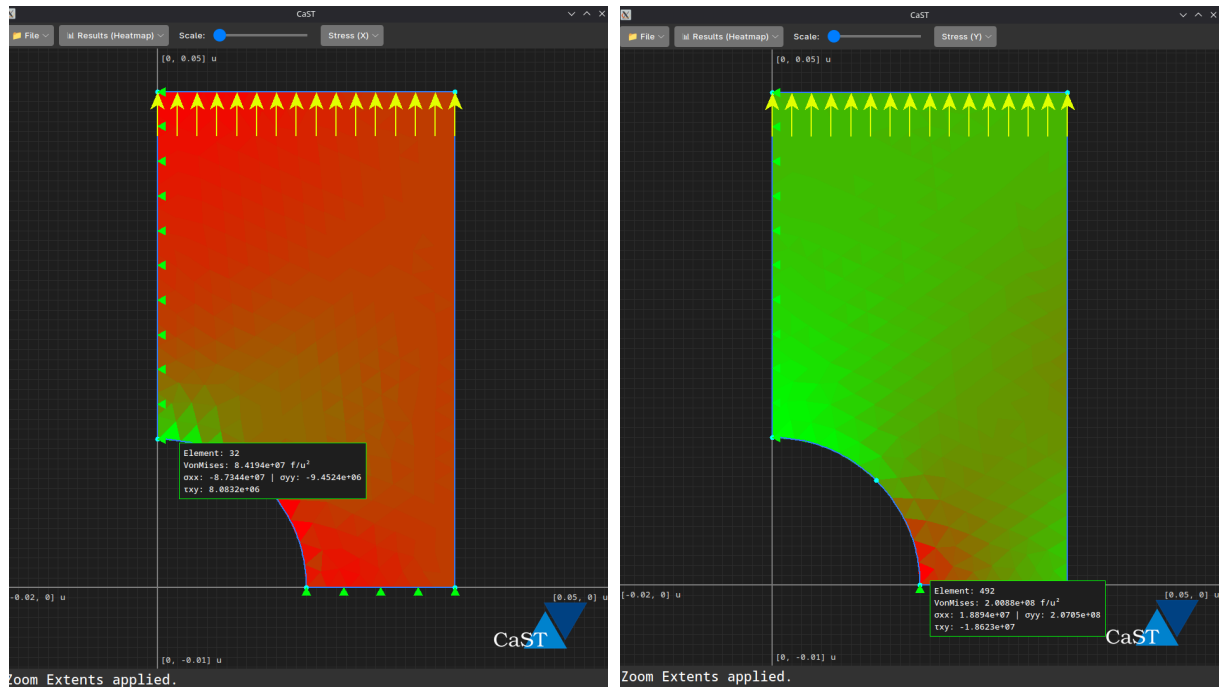
Figure 12: Stress heatmaps for x and y, respectively
