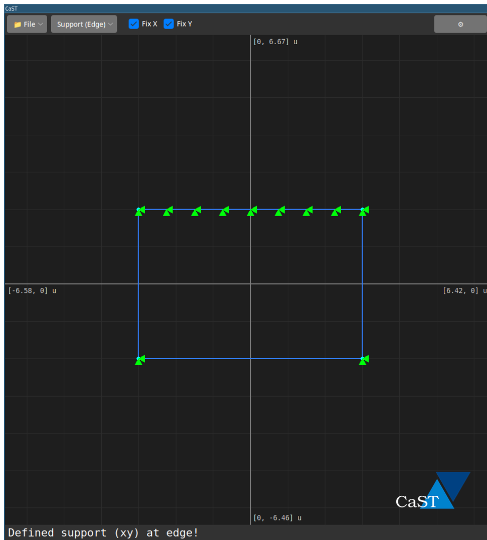
Figure 3: A rectangular object defined with supports at nodes (lower nodes) and edges (upper edge)
