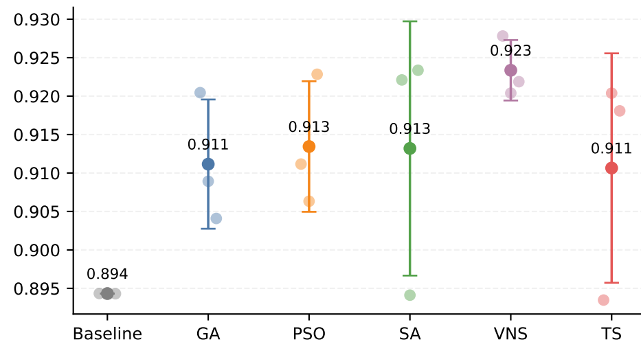
Selected features
