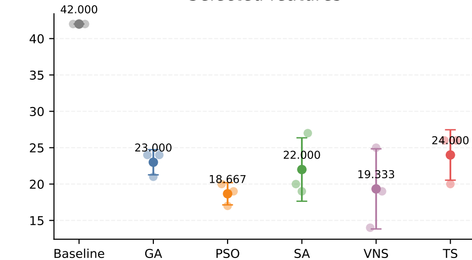
Selected features
