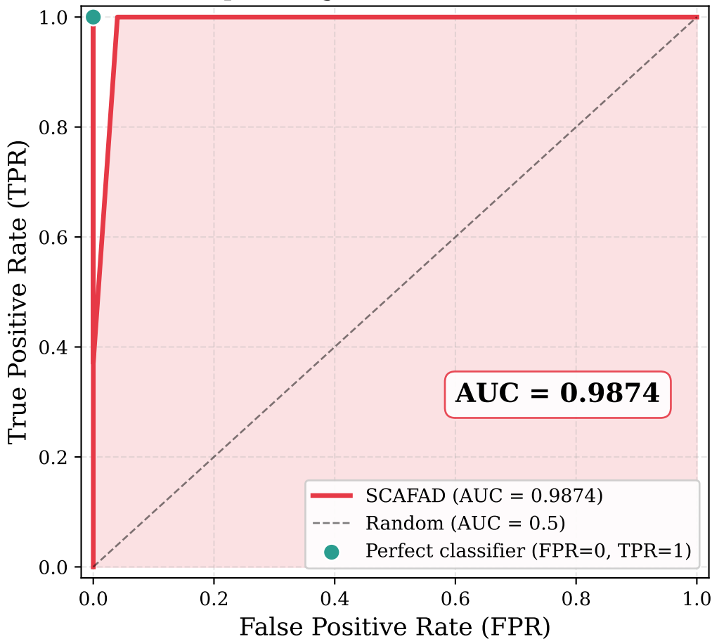
Receiver Operating Characteristic (ROC) Curve
