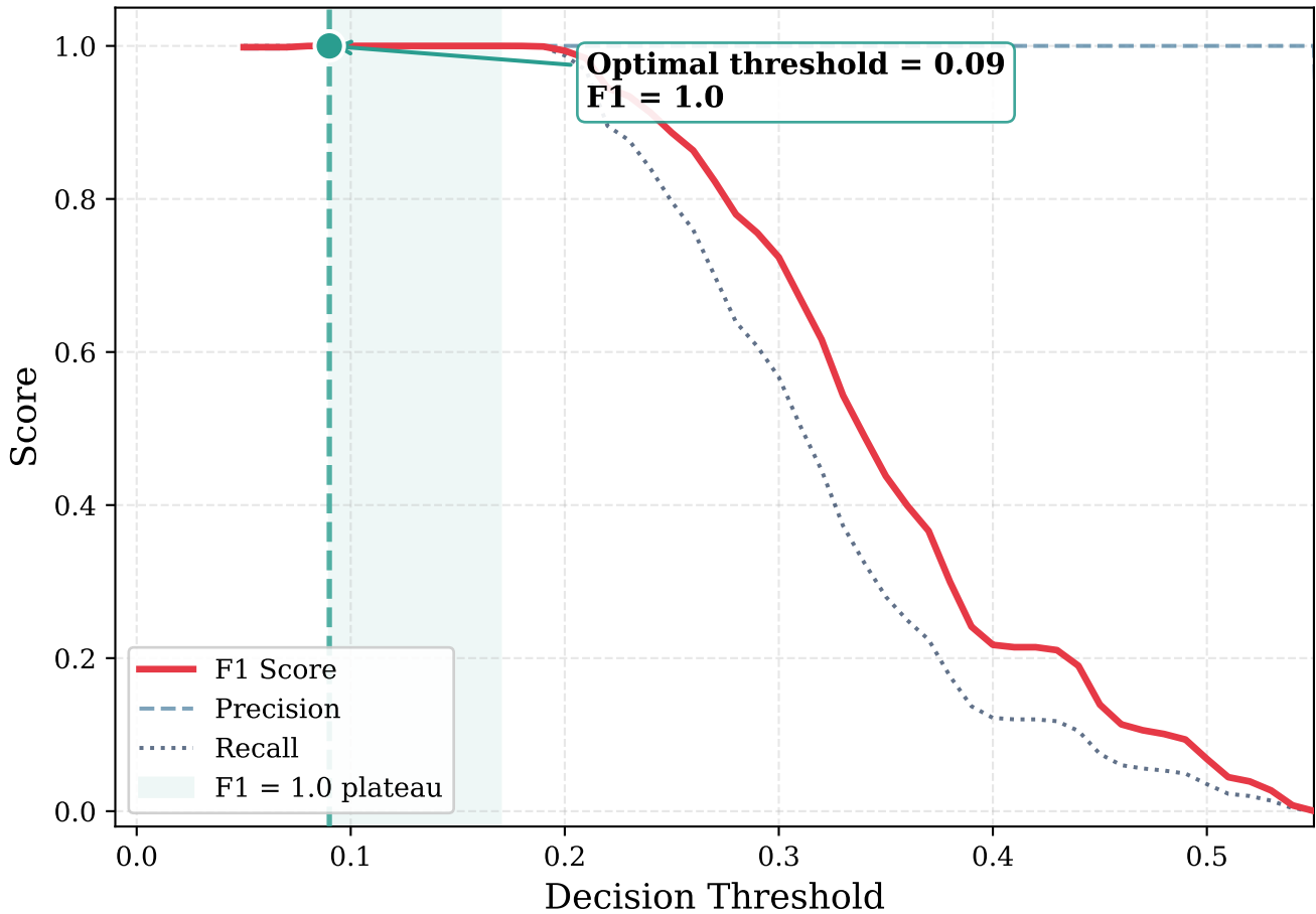
Threshold Grid Search — F1, Precision, and Recall vs Threshold
