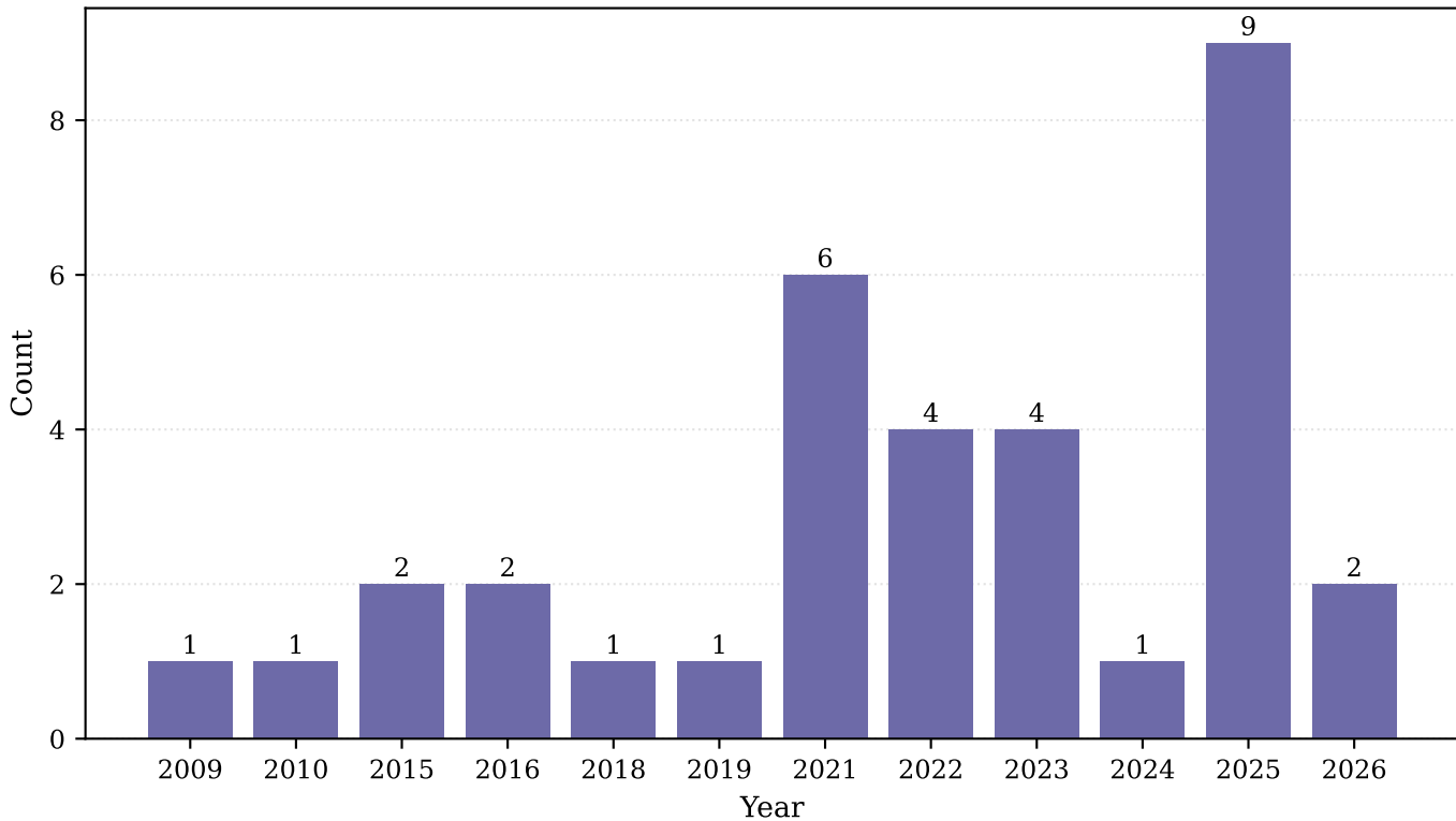
Publication-year distribution
