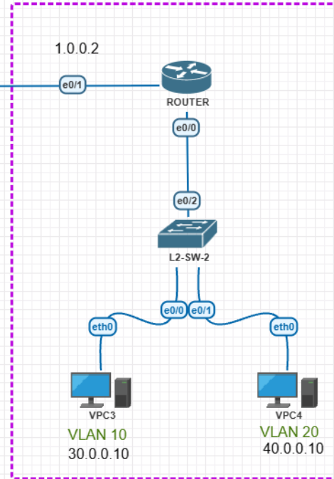
ROUTER ON-A-STICK
