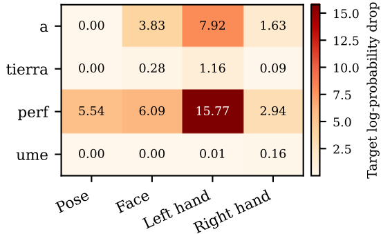
Region ablation
