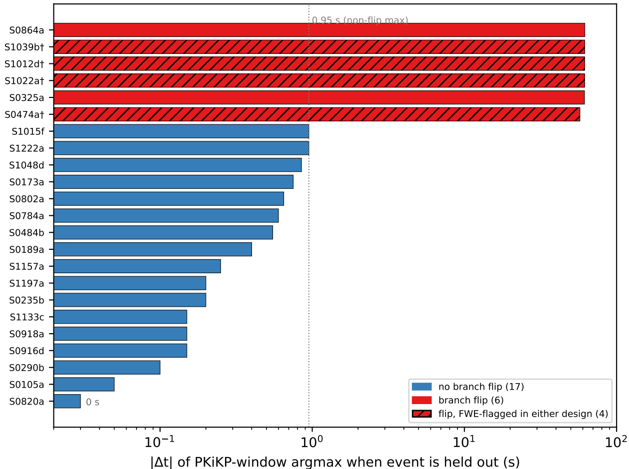
Leave-one-out influence, registered lane (23 events)
